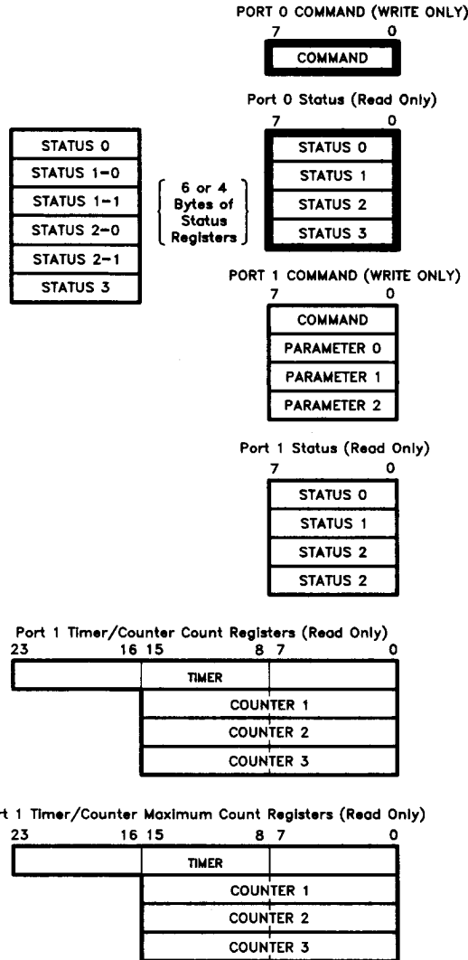
Figure 4. Programming Model—Directly Accessible Registers (Accessible Through 8-Bit I/O Port[s])
