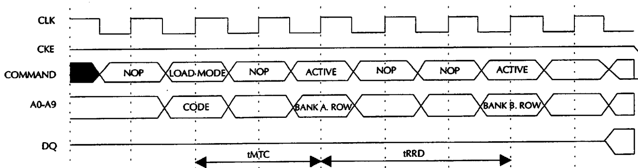
Figure 9.13 - SGRAM Timing
