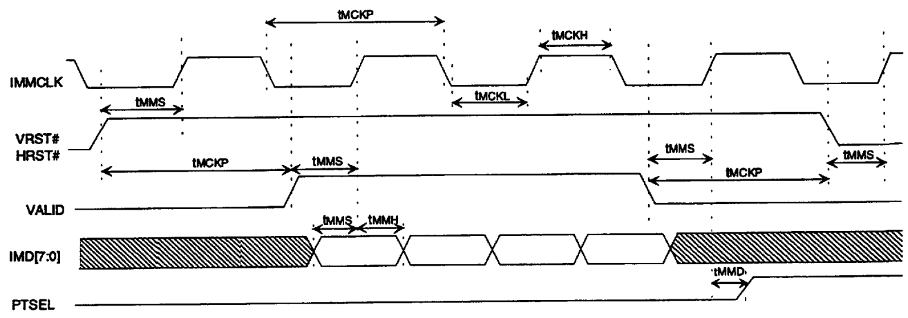
Figure 9.16 - 8-bit MediaBus Timing
