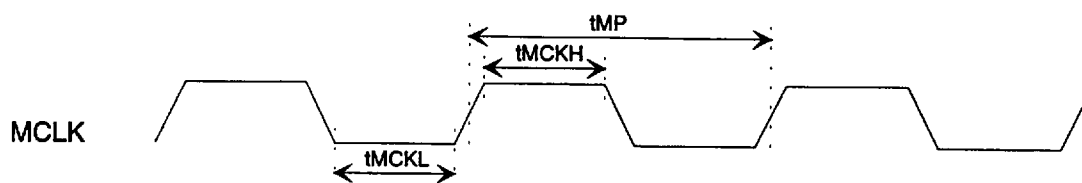
Figure 9.11 - Memory Clock Requirement
