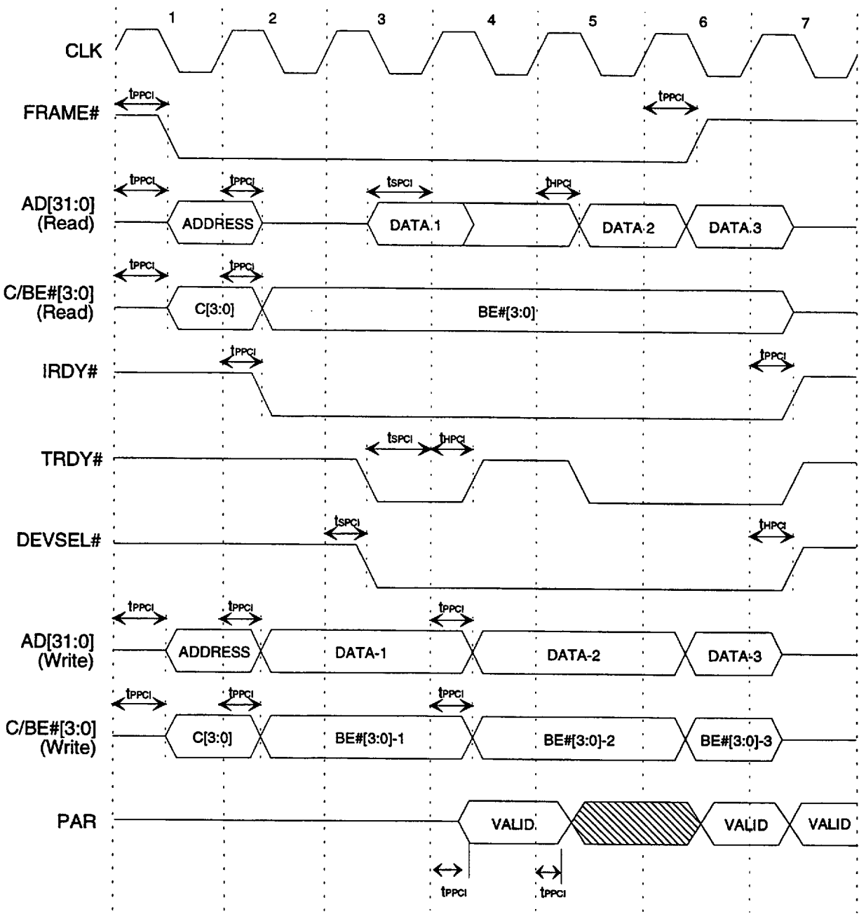
Figure 9.6 - PCI Bus Master Read/Write Timing
