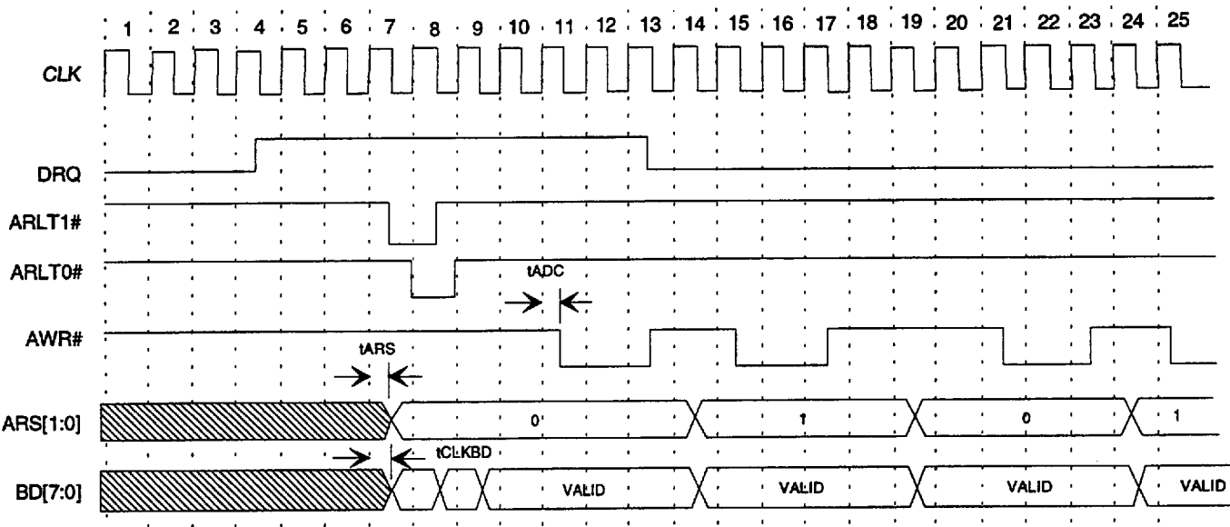
Figure 9.9 - DMA Transfer on AuxBus
