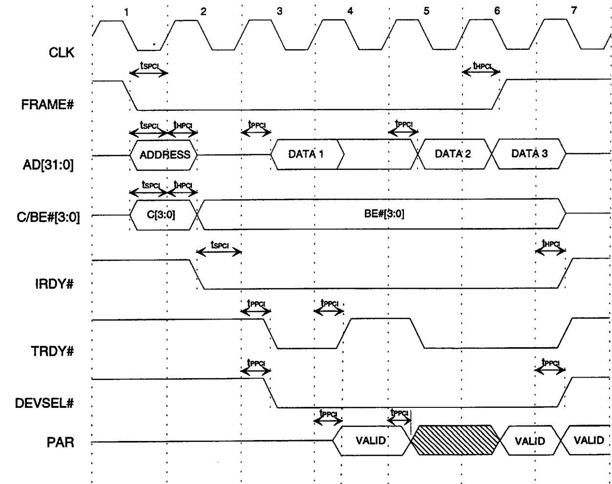
Figure 9.3 - PCI Bus Timing (Read Operation)
