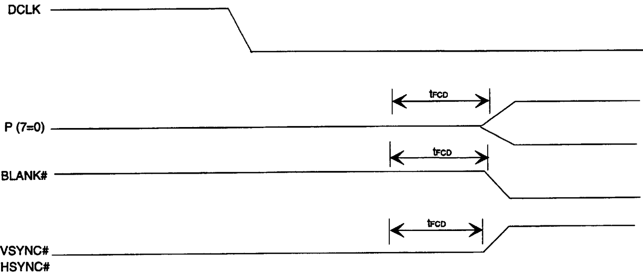
Figure 9.19 - Feature Connector Output Timing
