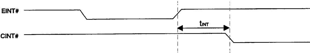
Figure 9.10 - Interrupt Timing
