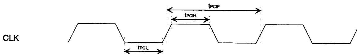
Figure 9.2 - PCI Bus Clock Requirement
