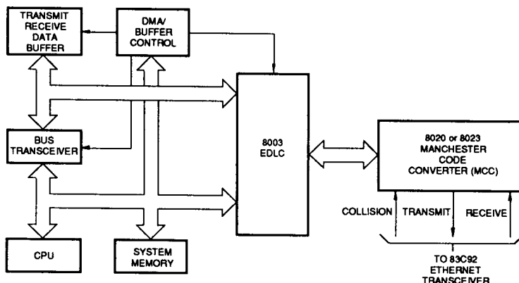
Figure 5. Typical Ethernet Node Configuration
