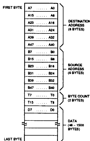
Figure 3. Typical Frame Buffer Format for Byte-Organized Memory
