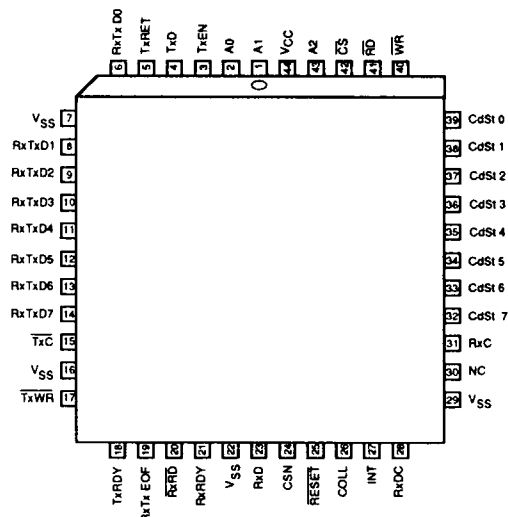
Figure 2. Plastic Leaded Chip Carrier Top view
