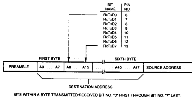
Figure 4. Bit Serialization/Deserialization
