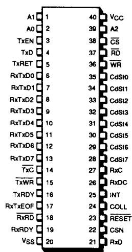
Figure 1. Dual-In-Line Top View
