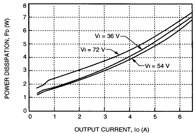
Figure 27. JW030F Power Dissipation vs. Output Current
