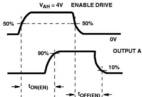
FIGURE 6A. t_{ON(EN)} , t_{OFF(EN)} MEASUREMENT
