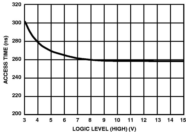
FIGURE 4A. ACCESS TIME vs LOGIC LEVEL (HIGH)
