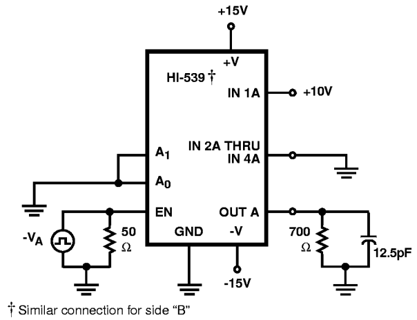
FIGURE 6B. t_{ON(EN)} , t_{OFF(EN)} TEST CIRCUIT
