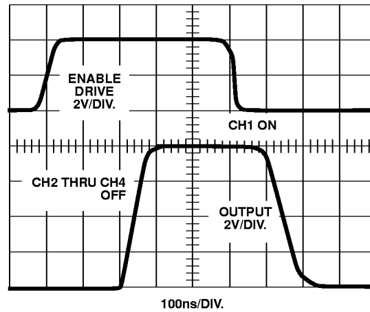
FIGURE 6C. t_{ON(EN)} , t_{OFF(EN)} WAVEFORMS
