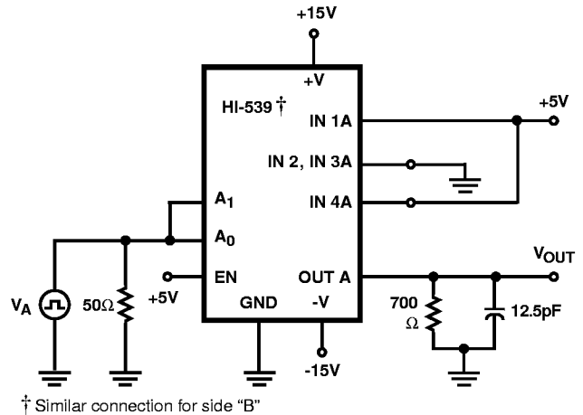
FIGURE 5B. t_{\text{OPEN}} TEST CIRCUIT
