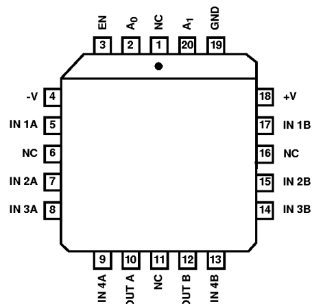
HI4P539 (PLCC) TOP VIEW
