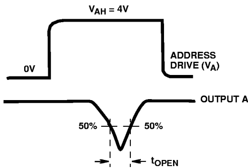
FIGURE 5A. t_{\text{OPEN}} MEASUREMENT
