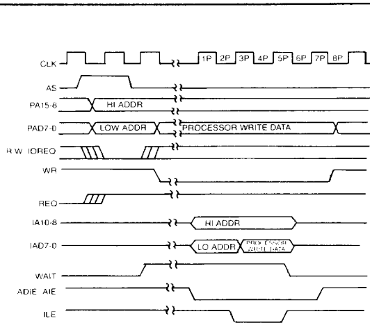
FIGURE 7—PROCESSOR WRITE COM 9026
