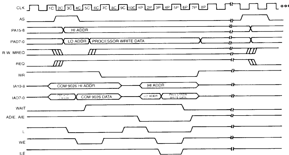
FIGURE 5—COM 9026 WRITE RAM FOLLOWED BY PROCESSOR WRITE RAM
