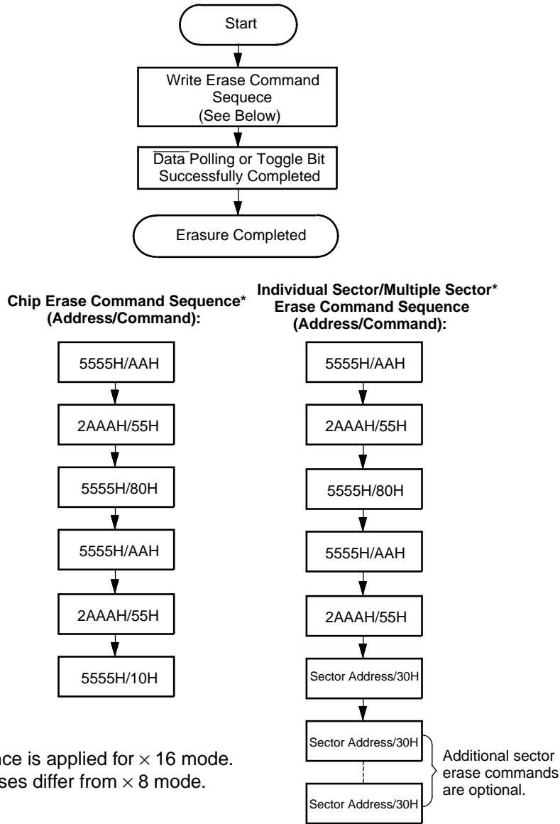
Figure 19 Embedded Erase Algorithm
