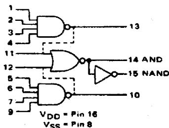
NTE4501 16-Lead DIP, See Diag. 249 Dual 4-Input NAND Gate, 2-Input NOR/OR Gate, 8-Input AND/NAND Gate
