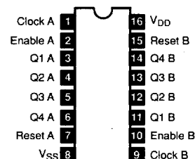
NTE4518B (BCD) NTE4520B (Binary) 16-Lead DIP, See Diag. 249 Dual Up/Down Counter
