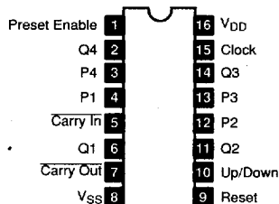
NTE4510B 16-Lead DIP, See Diag. 249 Presetable Up/Down BCD Counter
