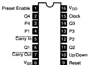
NTE4516B 16-Lead DIP, See Diag. 249 Presetable Up/Down Binary Counter
