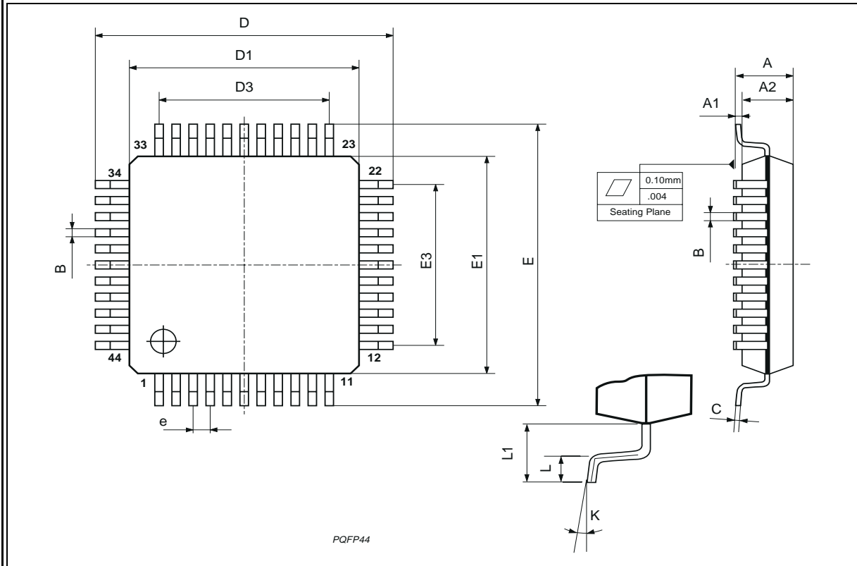
PQFP44 (10 x 10)
