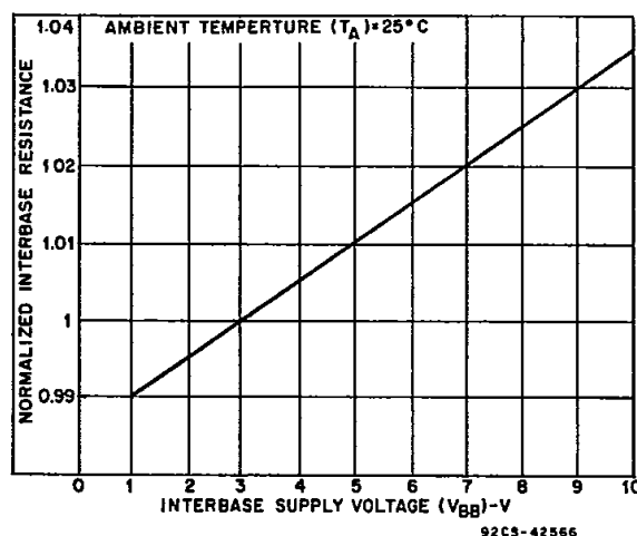
Fig. 13 - Normalized interbase resistance characteristic.
