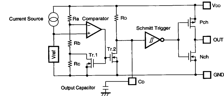
FIG. 1 Block Diagram
