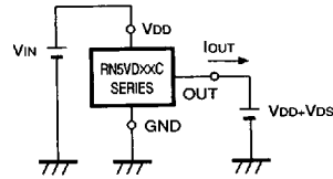
FIG. 6 Pch Driver Output Current Test Circuit
