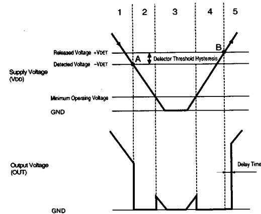
FIG. 2 Operation Diagram
