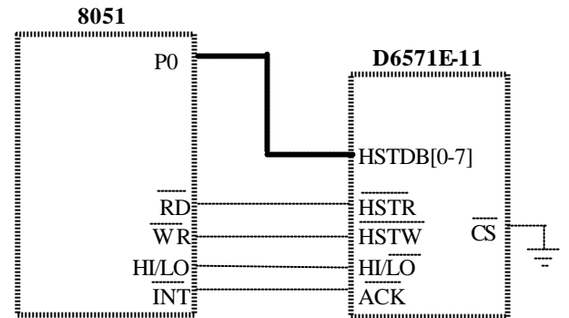
Figure 6. Host Interface D6571E - 8051
