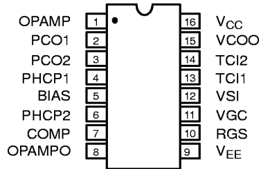
16 Pin PDIP
