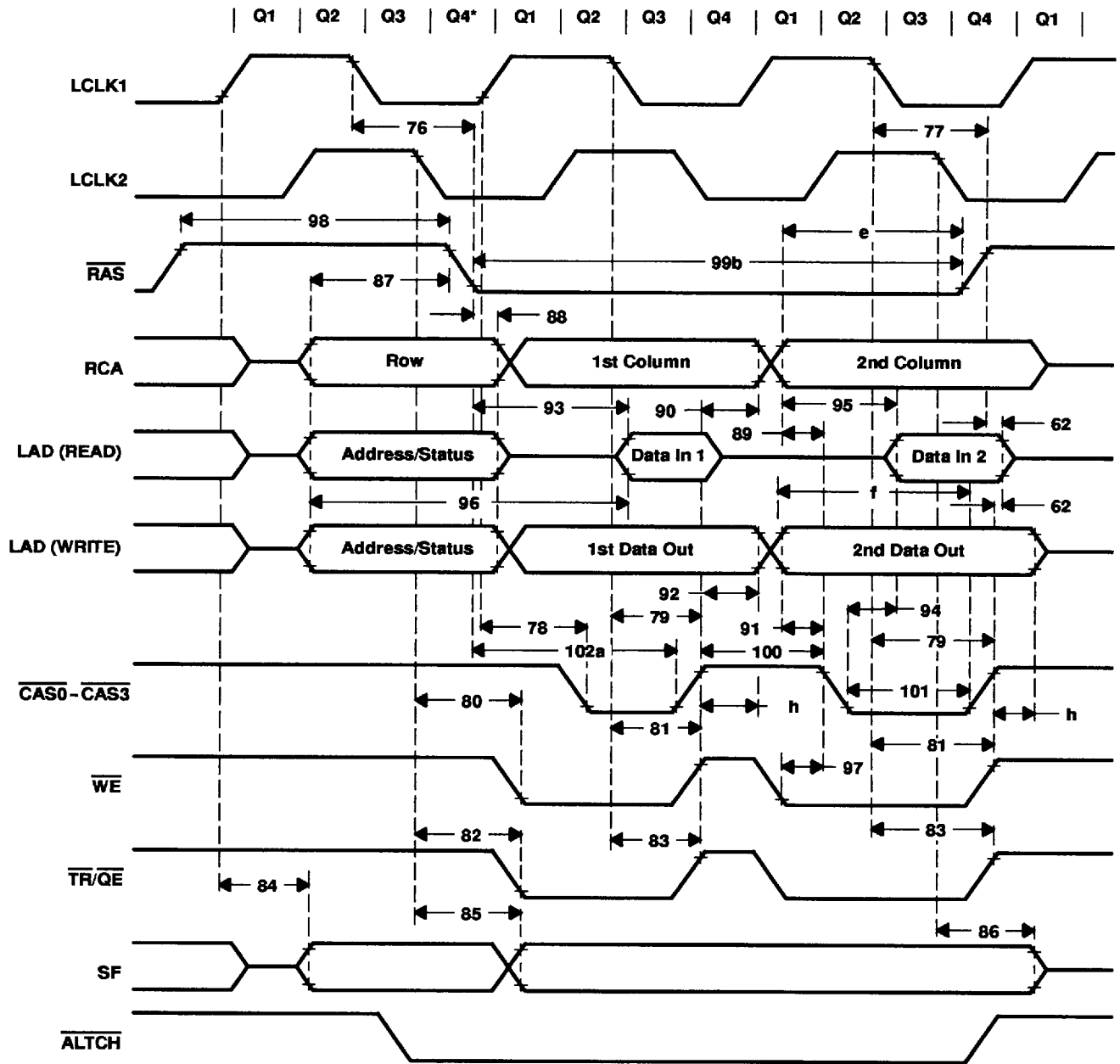
Figure 42. Local Bus Timing: \overline{\text{RAS}} , \overline{\text{CAS0-CAS3}} , \overline{\text{WE}} , \overline{\text{TR/QE}} , and SF
