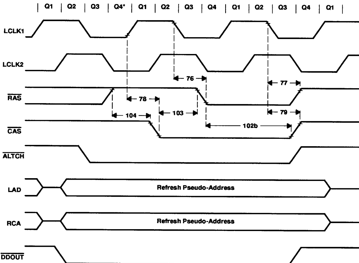
Figure 43. \overline{\text{CAS}} -Before- \overline{\text{RAS}} Refresh: \overline{\text{RAS}} and \overline{\text{CAS0}}-\overline{\text{CAS3}}
