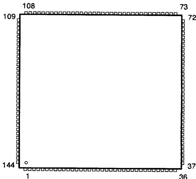
144-PIN PCM QUAD FLAT PACKAGE (TOP VIEW)
