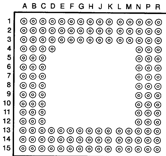
145-PIN GB PACKAGE (TOP VIEW)
