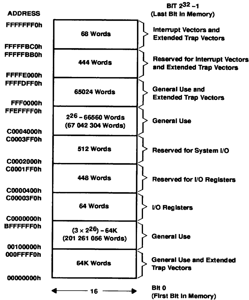
Figure 1. Memory Map
