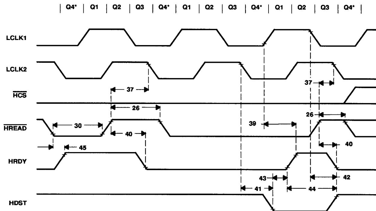
Figure 38. Host Interface Timing (Block Read Cycle)
