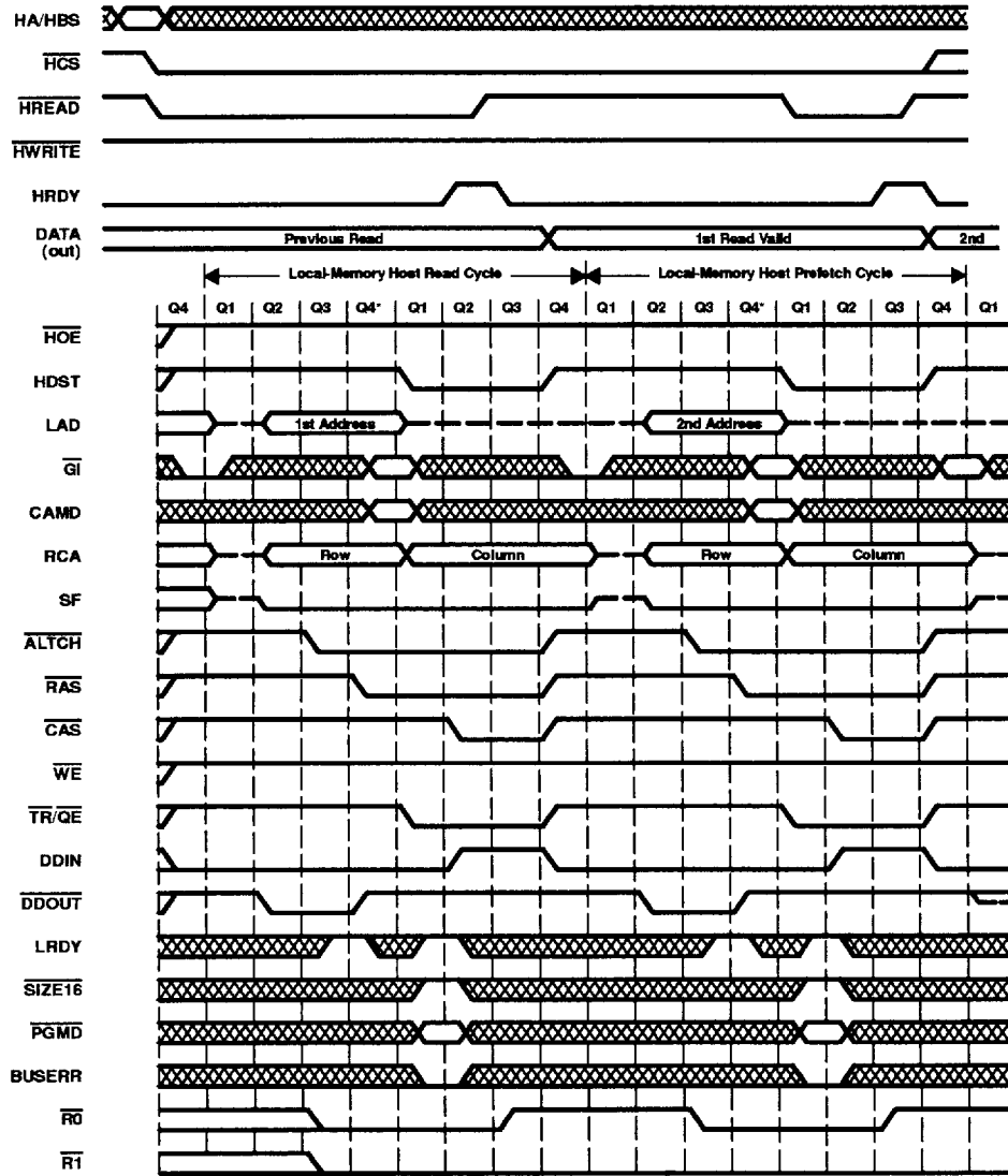
Figure 21. Back-to-Back Host Read Cycles With Implicit Addressing; \overline{\text{HREAD}} as Strobe
