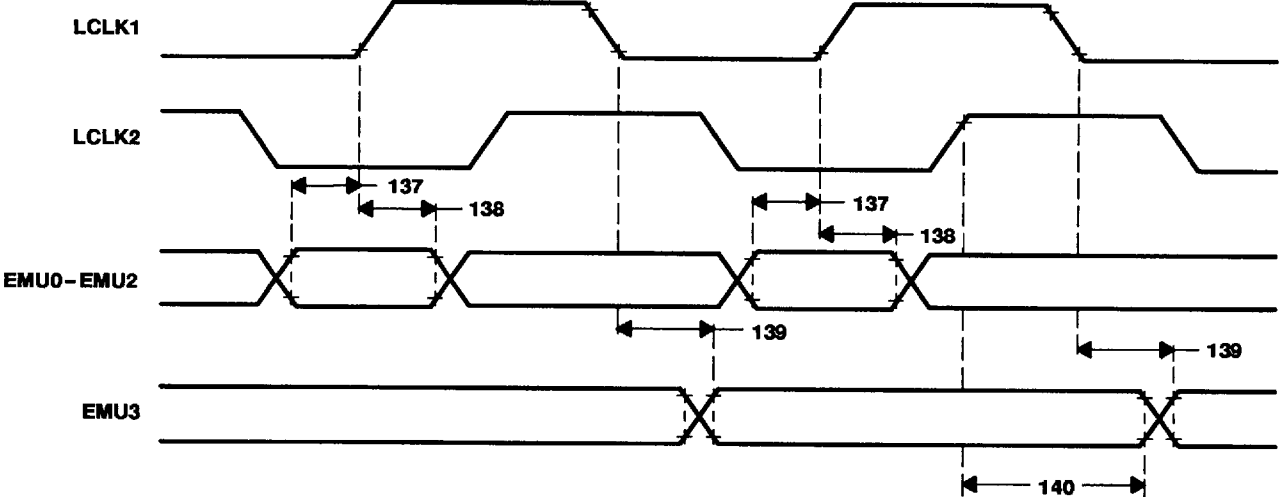
Figure 51. Emulator Interface Timing
