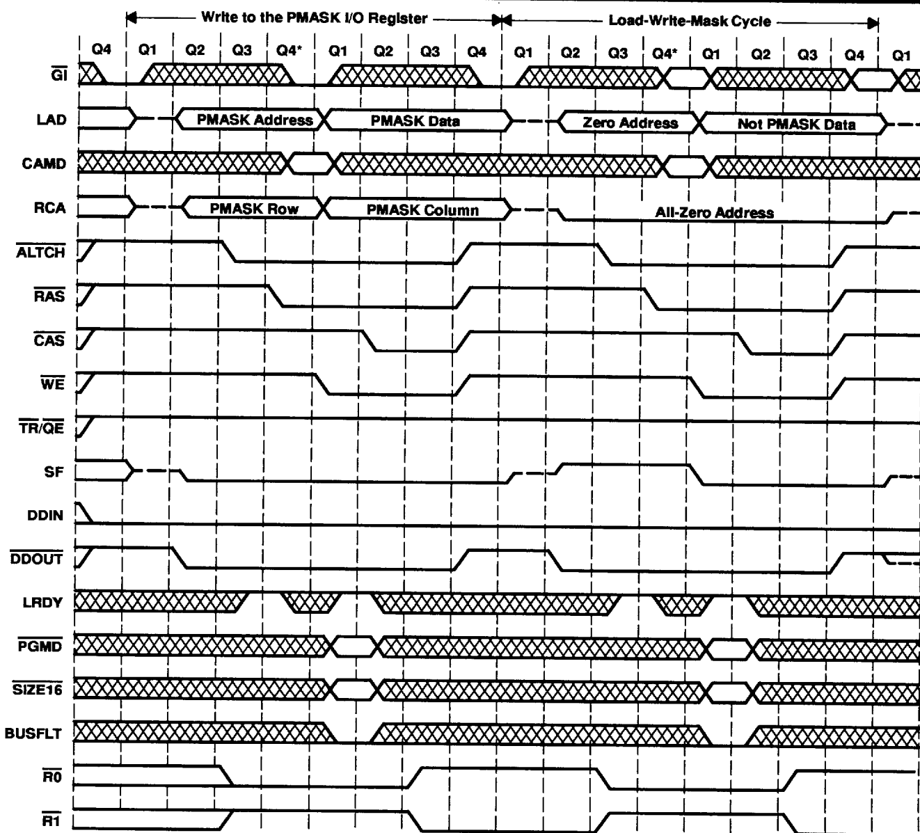
Figure 9. Load Write Mask Cycle
