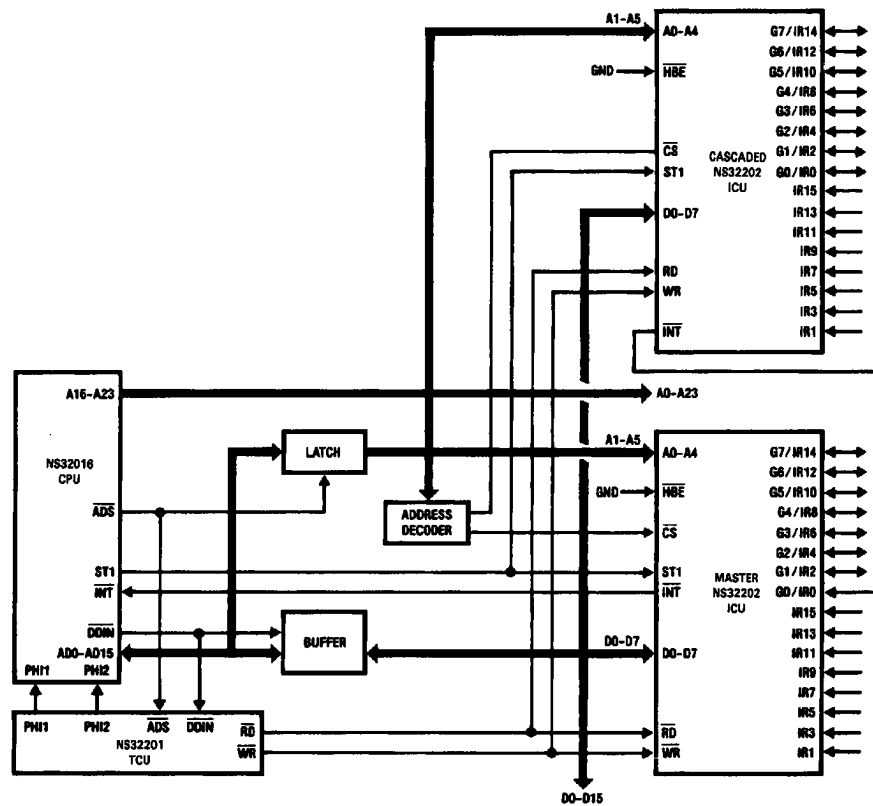
FIGURE 2-3. Cascaded Interrupt Control Unit Connections in 8-Bit Bus Mode
