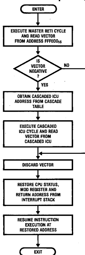
FIGURE 2-6. CPU Return from Interrupt Sequence
