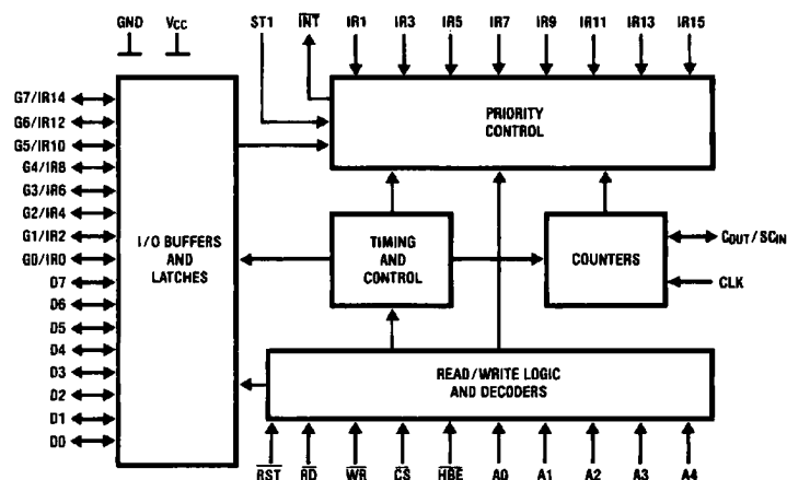
FIGURE 1-1. NS32202 ICU Block Diagram
