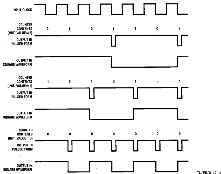
FIGURE 1-2. Counter Output Signals in Pulsed Form and Square Waveform for Three Different Initial Values
