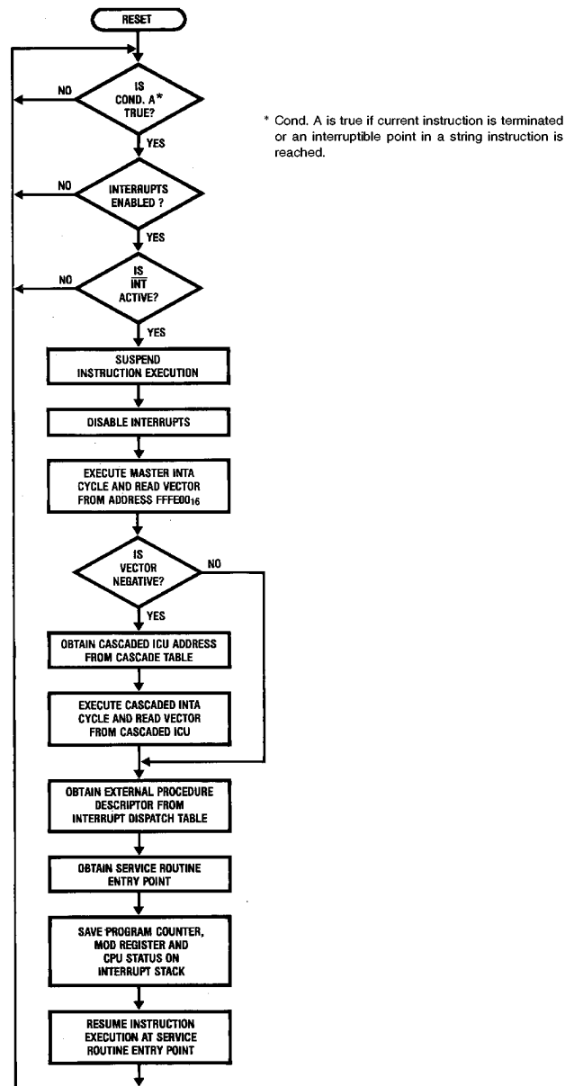
FIGURE 2-4. CPU Interrupt Acknowledge Sequence
