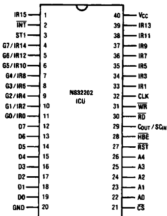
Top View Order Number NS32202D-10 See NS Package Number D40C
