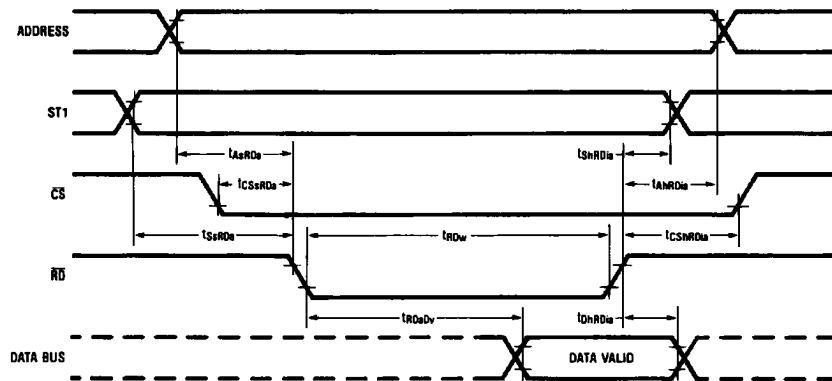
FIGURE 4-3. READ/INTA Cycle
