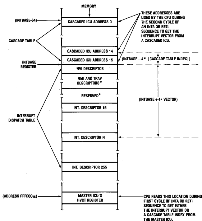
FIGURE 2-5. Interrupt Dispatch and Cascade Tables
