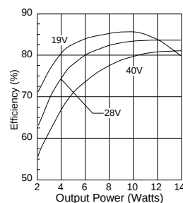
HR121-2815 Efficiency FIGURE 4
