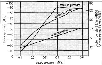
Flow Characteristics
