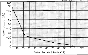
Flow Characteristics
