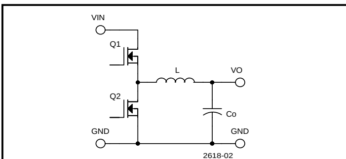
Fig. 2. Output filter components
