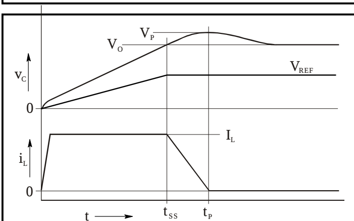
Fig. 3. Soft start, inductor current and overshoot
