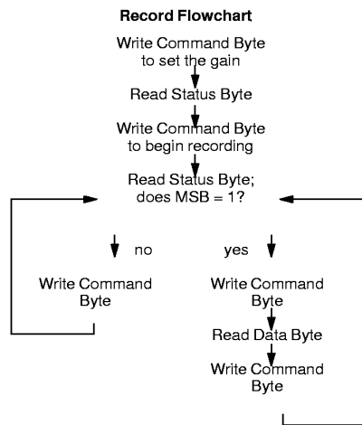
RECORD AND PLAYBACK FLOWCHARTS Figure 7
