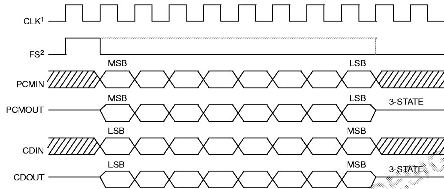
CD AND PCM PORT I/O DIAGRAM Figure 3
