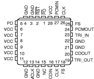
DS2132AQ 28-PIN PLCC
