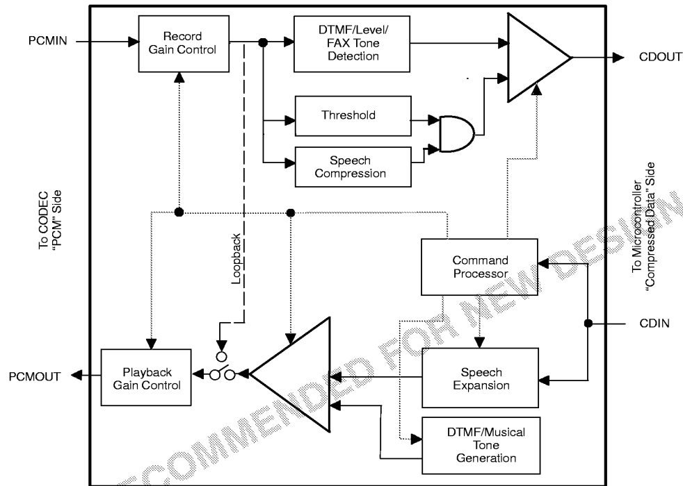
DS2132A BLOCK DIAGRAM Figure 2
