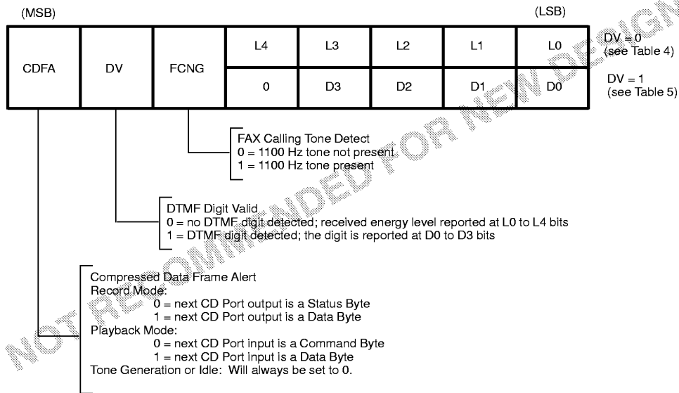
STATUS BYTE FORMAT Figure 6
