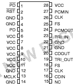
DS2132A 28-PIN DIP 600 MIL
