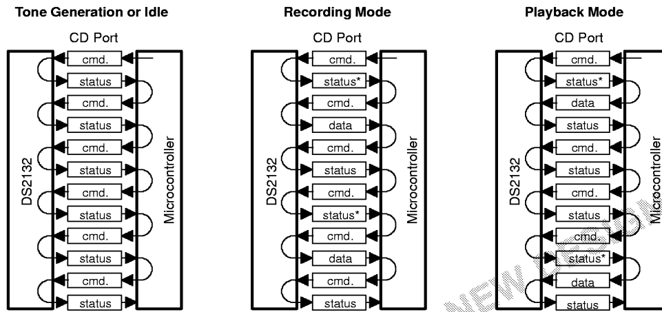
CD PORT FLOW STRUCTURE Figure 4
