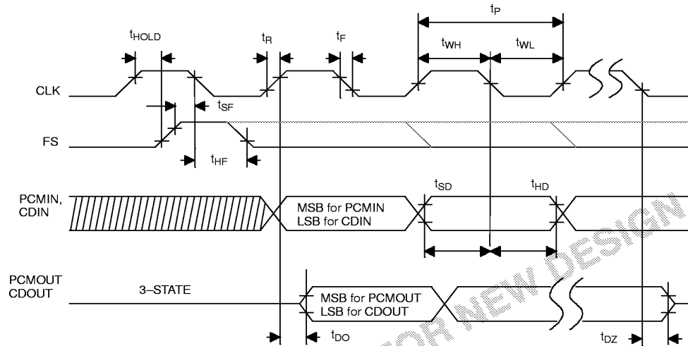
DATA I/O AC TIMING DIAGRAM Figure 8
