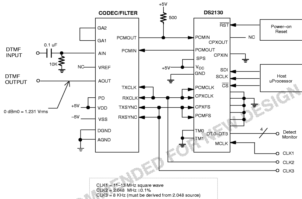
DTMF RECEIVER/GENERATOR TEST CIRCUIT Figure 12
