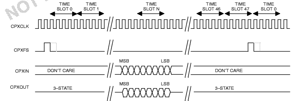
DS2130 CPX-SIDE INTERFACE Figure 8
