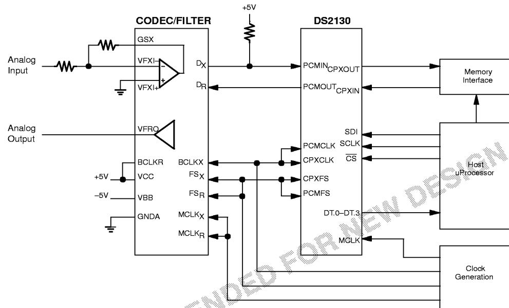
DS2130 CONNECTION TO CODEC/FILTER Figure 9
