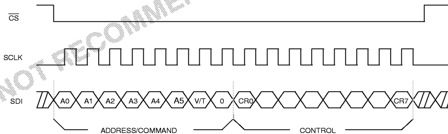
SERIAL PORT WRITE Figure 2
