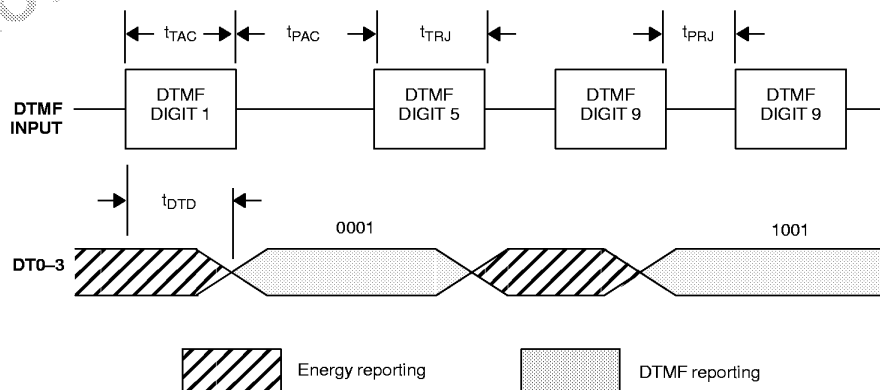
DTMF RECEIVER TIMING Figure 13
