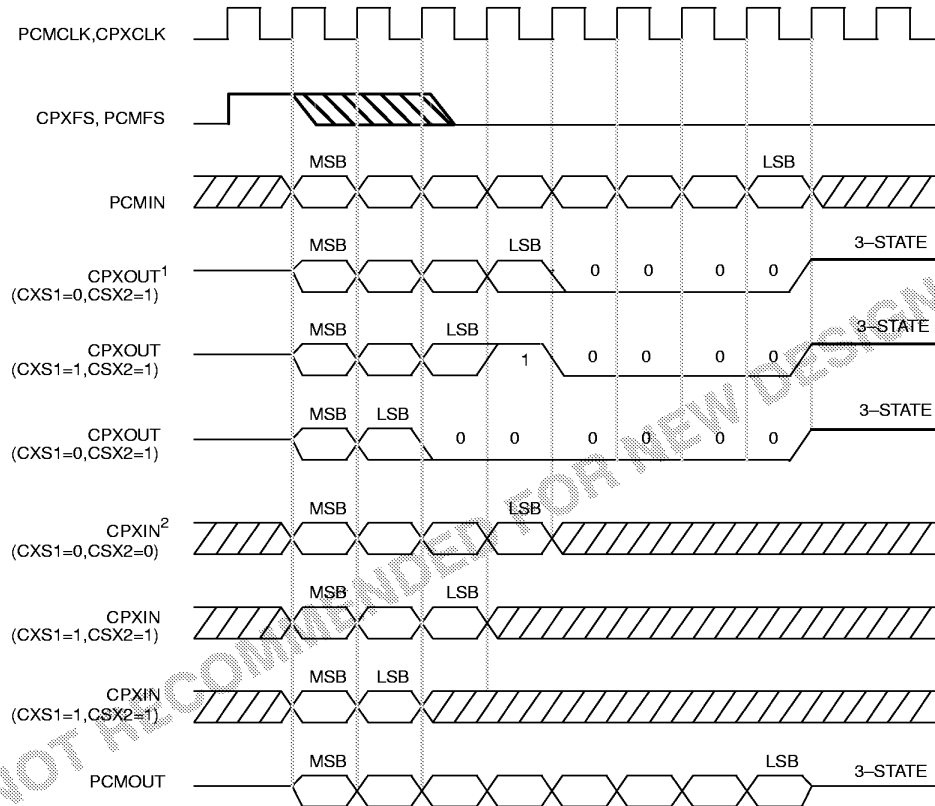
PCM/CPX I/O (CXS3=1) Figure 11
