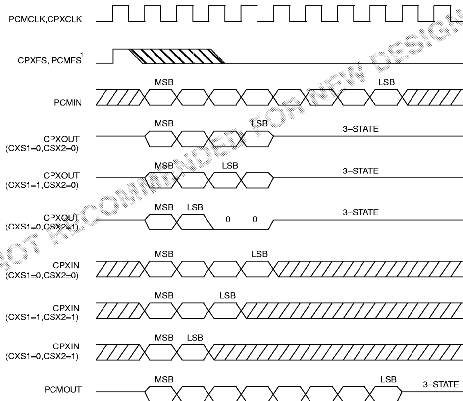
PCM/CPX I/O (CXS3=0) Figure 10
