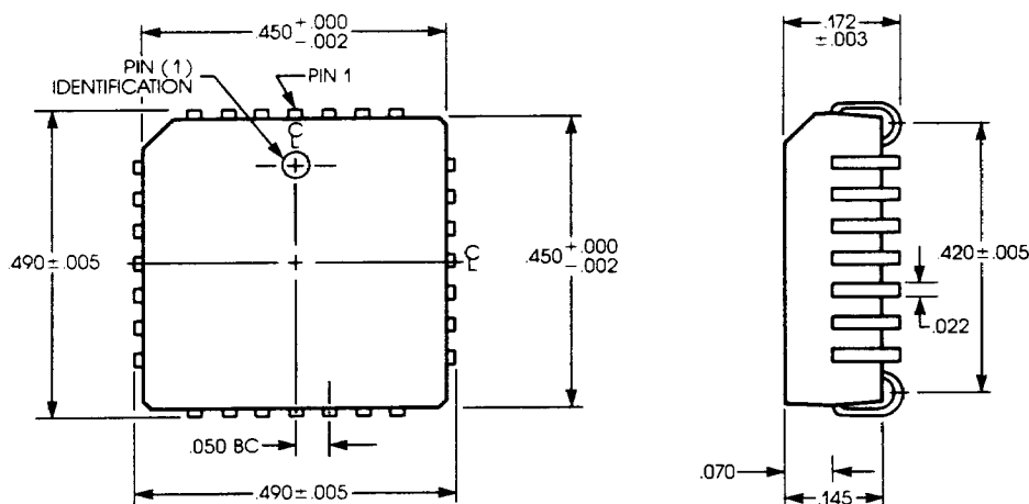
28-Lead Plastic Surface Mount Package
