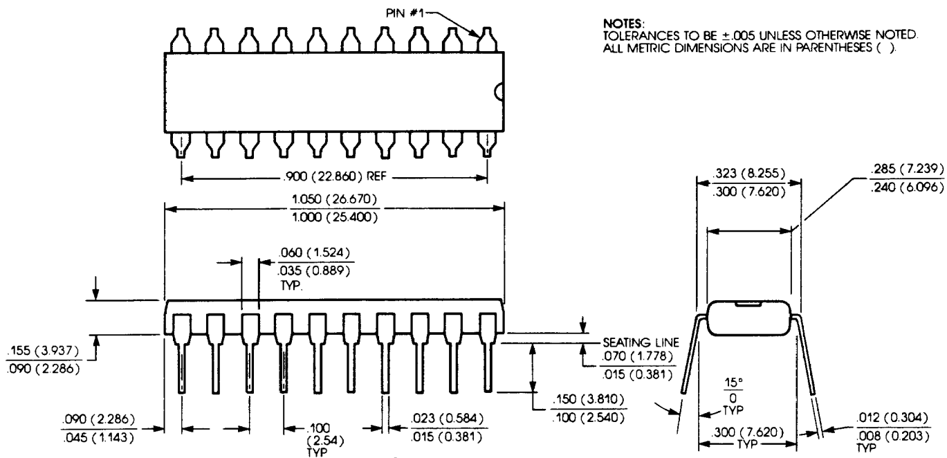
20-Pin Plastic Package Outline
