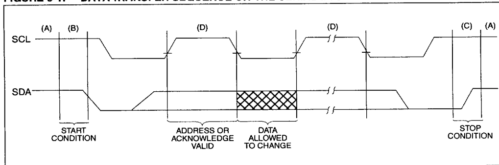
FIGURE 3-1: DATA TRANSFER SEQUENCE ON THE SERIAL BUS
