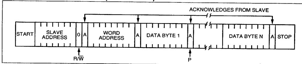
FIGURE 6-1: PROGRAM MODE (ERASE/WRITE)
