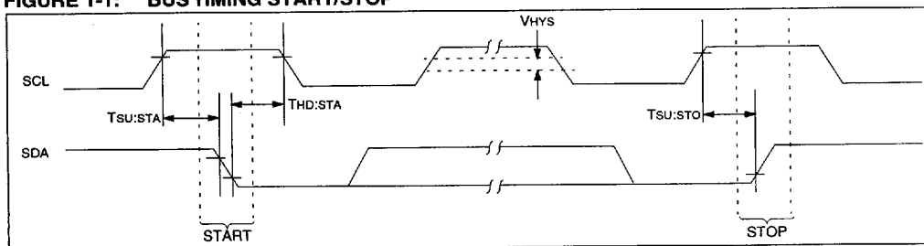
FIGURE 1-1: BUSTIMING START/STOP
