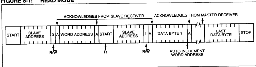
FIGURE 8-1: READ MODE
