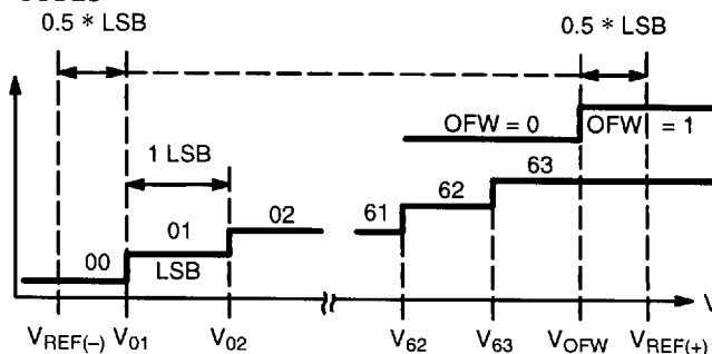
Figure 8. Ideal A/D Transfer Function
