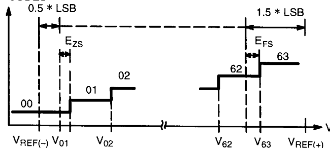
Figure 9. Real A/D Transfer Curve
