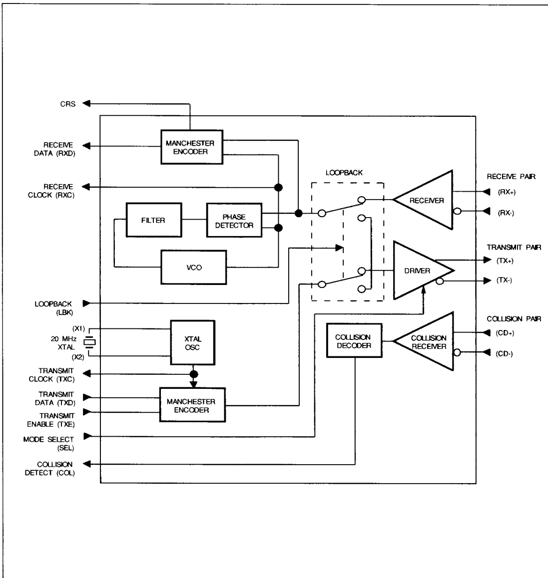
FIGURE 2-1. WD83C691A GENERAL SYSTEM BLOCK DIAGRAM
