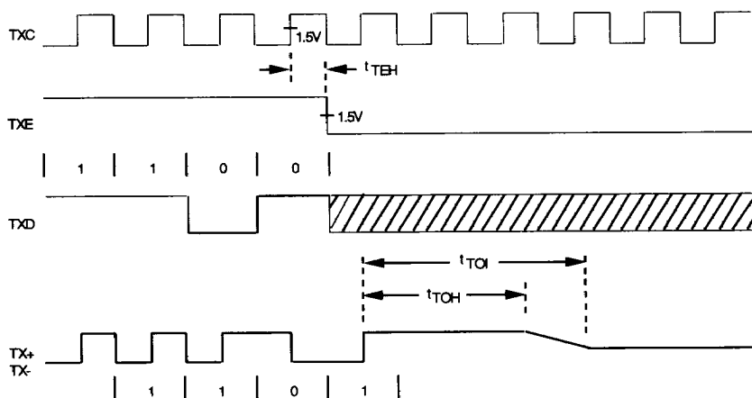
FIGURE C-3. TRANSMIT TIMING - TRANSMISSION END (LAST BIT=1)
