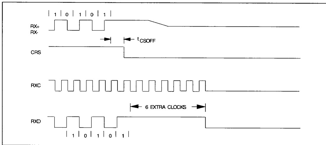
FIGURE C-6. RECEIVE TIMING - END OF PACKET (LAST BIT = 1)
