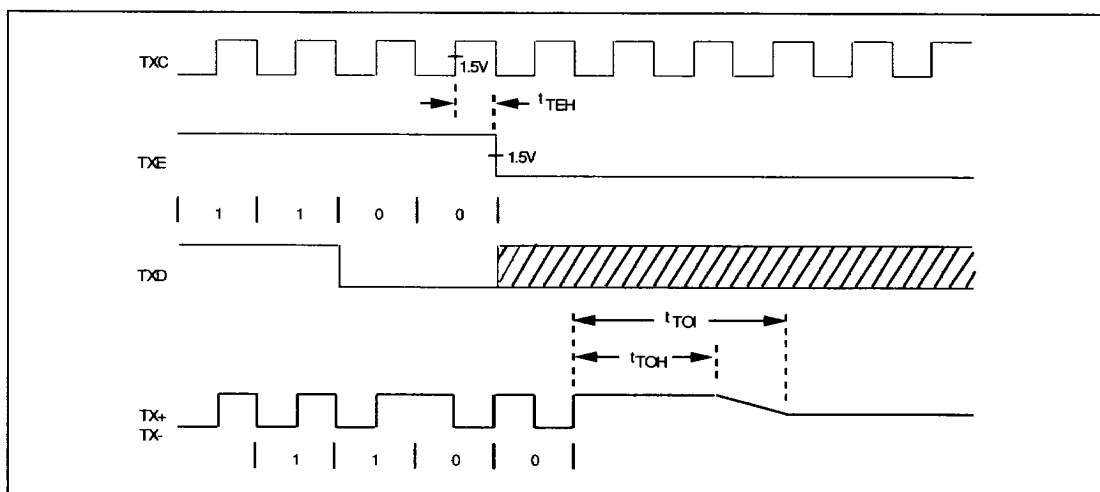
FIGURE C-2. TRANSMIT TIMING - TRANSMISSION END (LAST BIT=0)
