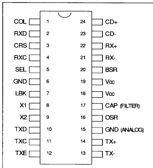
FIGURE A-1. WD83C691-PG 24-Pin DIP Manchester Encoder/Decoder
