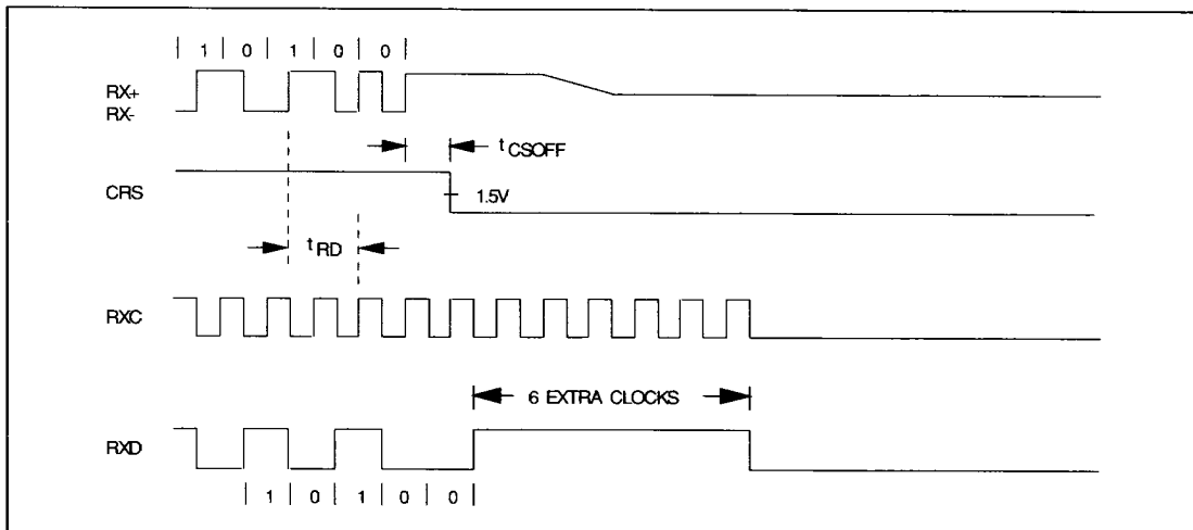
FIGURE C-5. RECEIVE TIMING - END OF PACKET (LAST BIT = 0)
