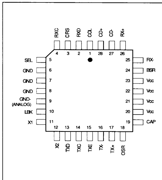
FIGURE A-2. WD83C691-JH 28-Pin PLCC Manchester Encoder/Decoder
