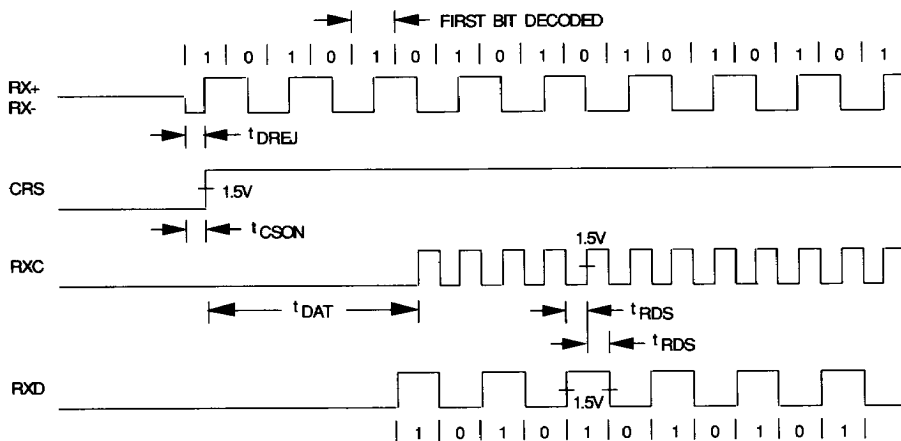
FIGURE C-4. RECEIVE TIMING - START OF PACKET
