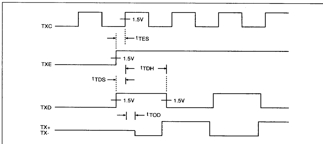
FIGURE C-1. TRANSMIT TIMING - TRANSMISSION START
