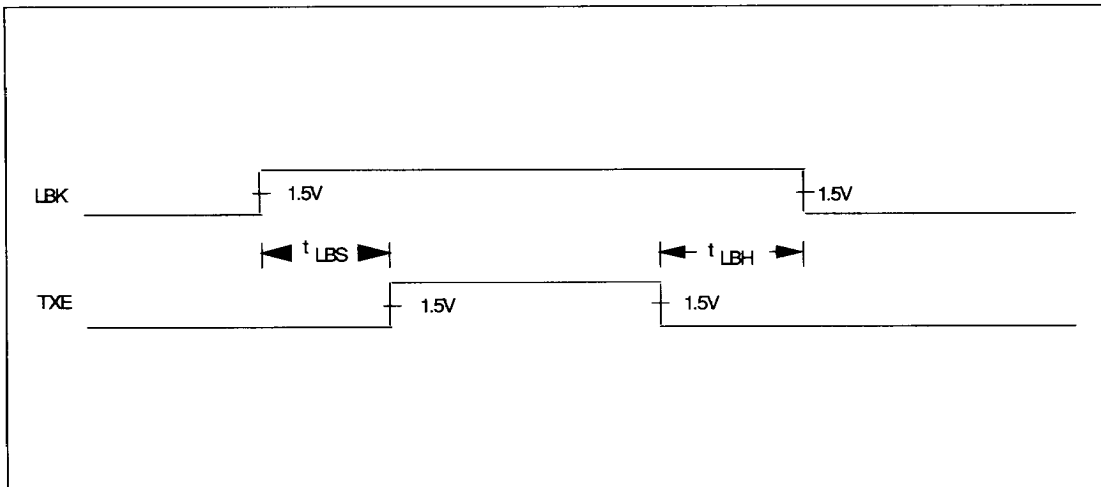
FIGURE C-8. LOOPBACK TIMING
