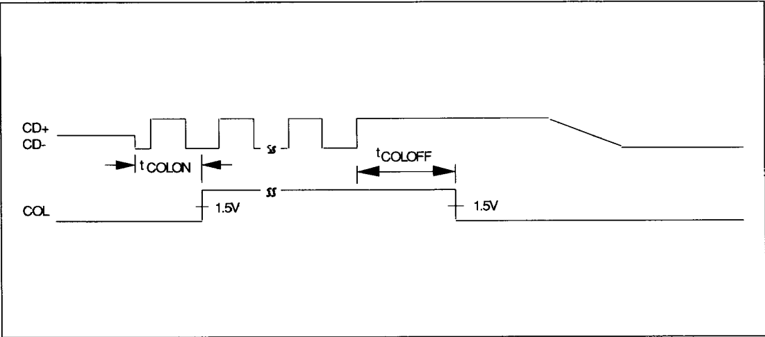
FIGURE C-7. COLLISION TIMING
