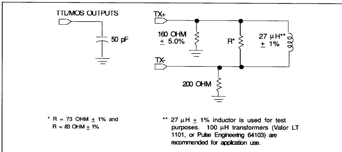
FIGURE C-9. TEST LOADS
