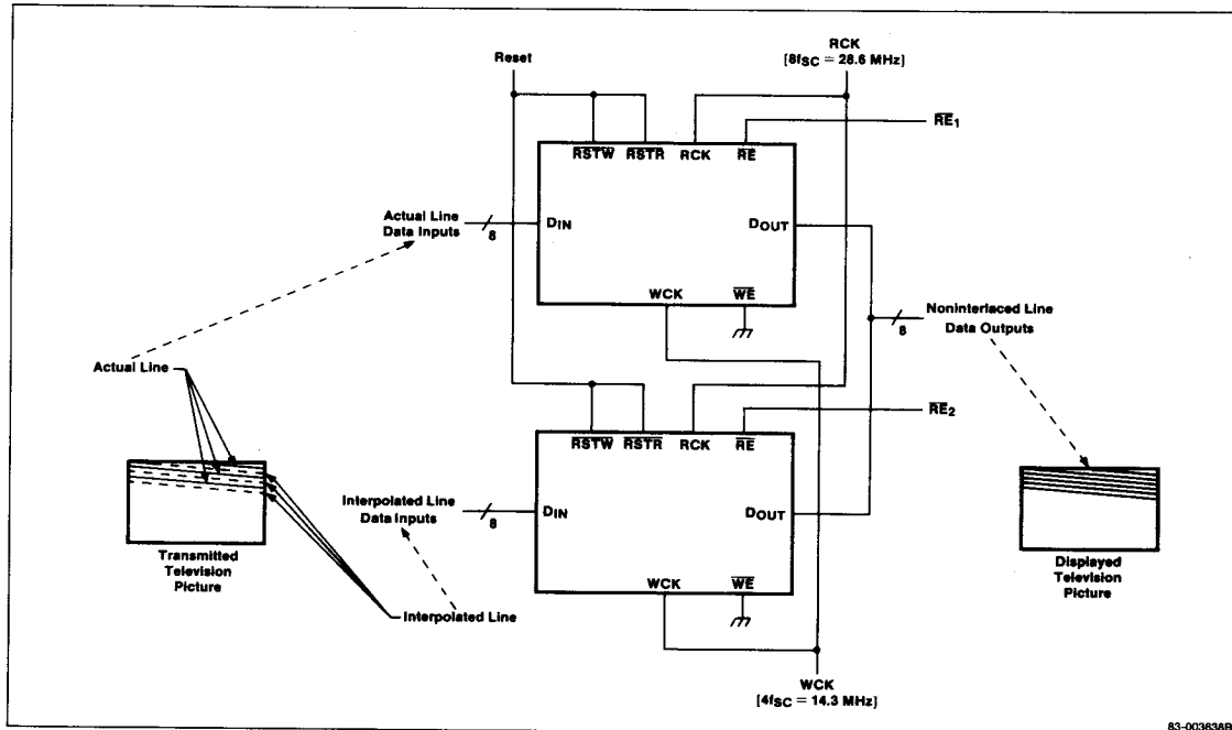
Figure 1. Connection for Noninterfaced Scan Conversion
