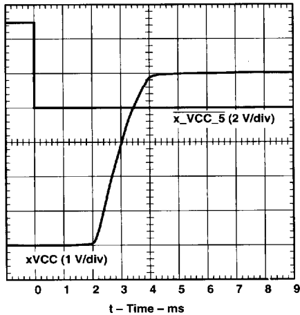
Figure 8. xVCC Propagation Delay and Rise Times With 100- \mu F Load, 5-V Switch
