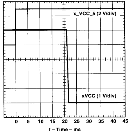
Figure 7. xVCC Propagation Delay and Fall Times With 1- \mu F Load, 5-V Switch
