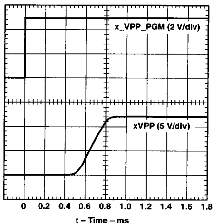
Figure 10. xVPP Propagation Delay and Rise Times With 1- \mu F Load, 12-V Switch
