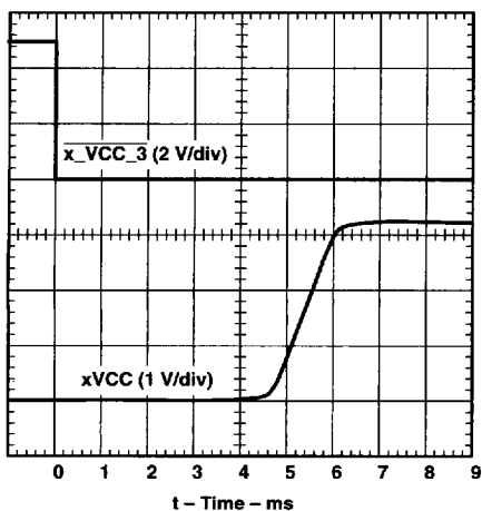
Figure 4. xVCC Propagation Delay and Rise Times With 100- \mu F Load, 3-V Switch
