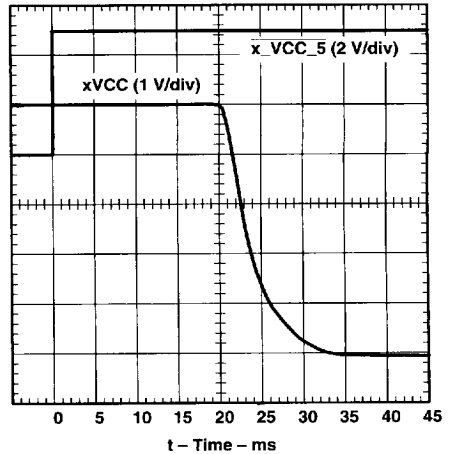
Figure 9. xVCC Propagation Delay and Fall Times With 100- \mu F Load, 5-V Switch
