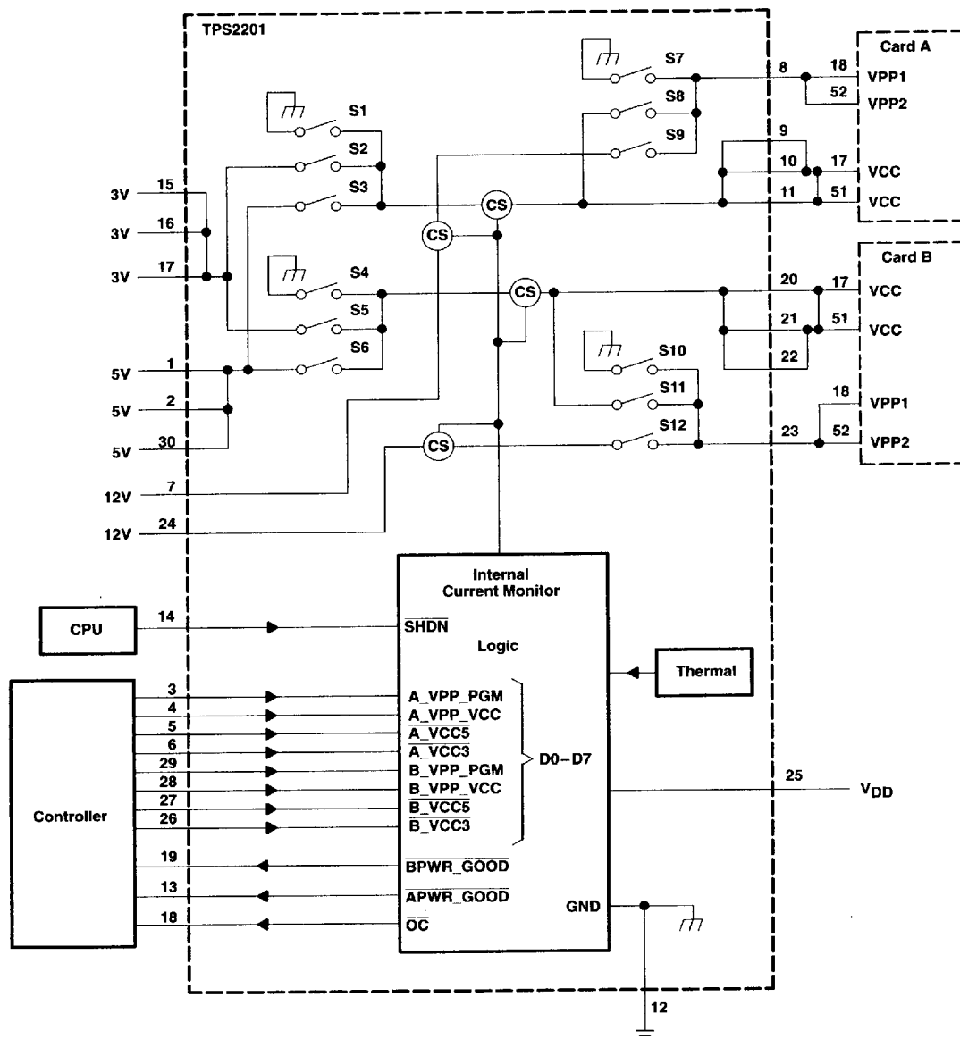
Figure 23. Internal Switching Matrix
