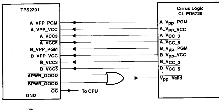
Figure 24. Logic Connections to CL-PD6720
