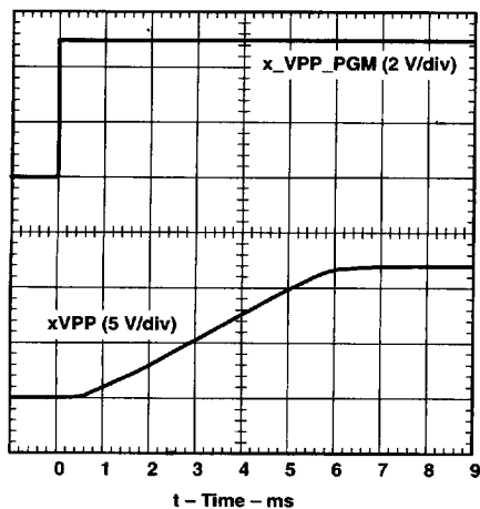
Figure 12. xVPP Propagation Delay and Rise Times With 100- \mu F Load, 12-V Switch
