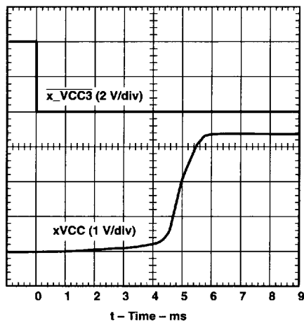
Figure 2. xVCC Propagation Delay and Rise Times With 1- \mu F Load, 3-V Switch
