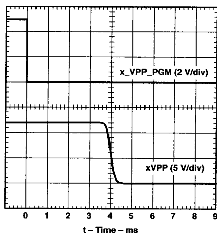
Figure 11. xVPP Propagation Delay and Fall Times With 1- \mu F Load, 12-V Switch
