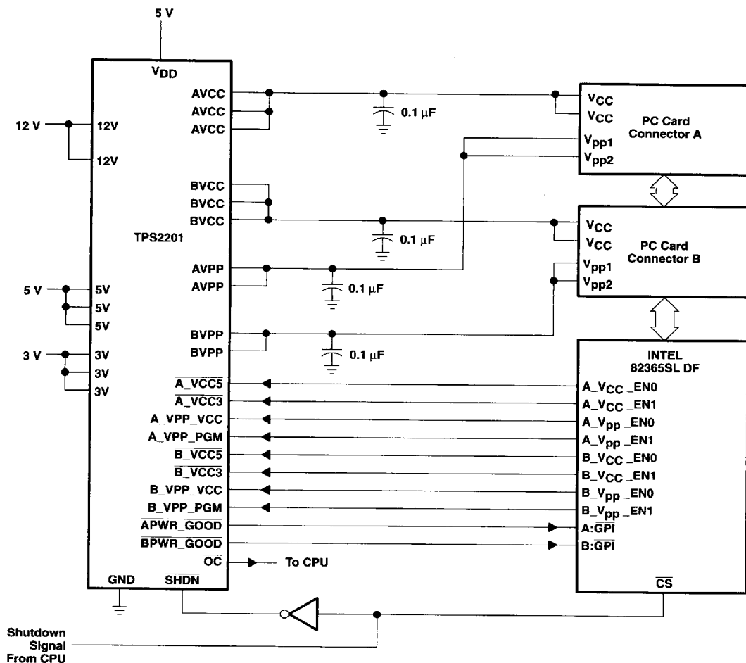
Figure 25. Detailed Operating Circuits Using Intel 82365SLDF Controller
