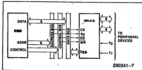
Figure 1. 8085A-8741A Interface
