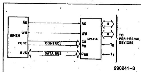
Figure 2. 8048-8741A Interface
