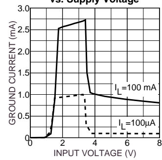
Ground Current vs. Supply Voltage
