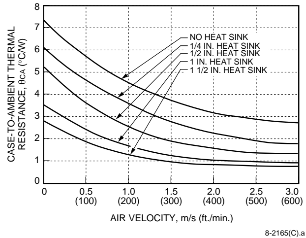
Figure 24. Case-to-Ambient Thermal Resistance Curves; Transverse Orientation
