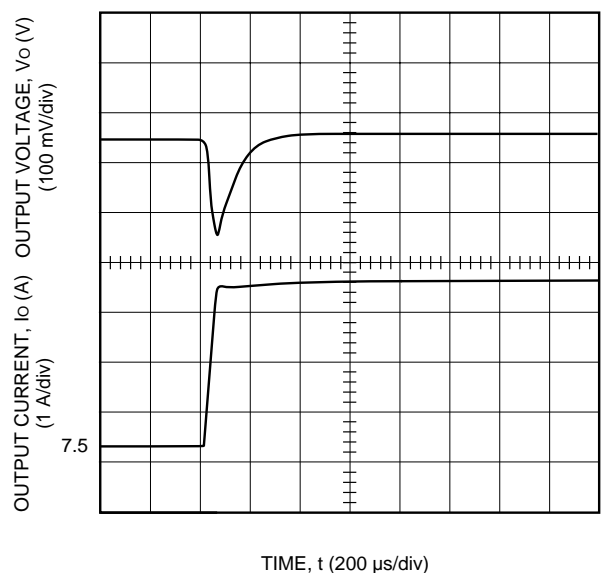
Figure 6. Typical JAW075A1 Transient Response to Step Increase in Load from 50% to 75% of Full Load at Room Temperature and 48 Vdc Input (Waveform Averaged to Eliminate Ripple Component.)
