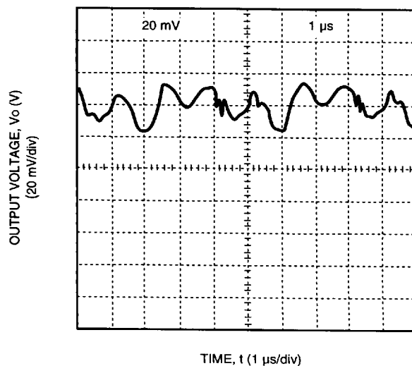
Figure 4. Typical FE150F Output Ripple Voltage at Room Temperature, 48 V Input, and 30 A Output
