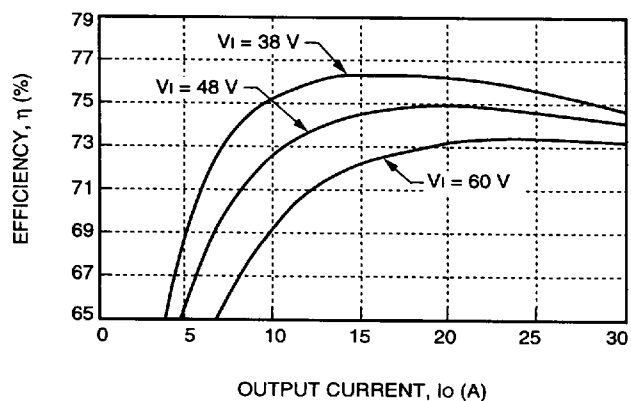
Figure 3. Typical FE150F Efficiency vs. Output Current at Room Temperature
