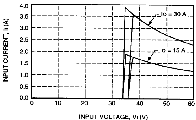
Figure 1. Typical FE150F Input Characteristics at Room Temperature
