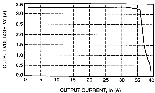
Figure 2. Typical FE150F Output Characteristics at Room Temperature and 48 V Input
