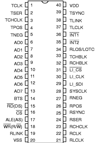
40-PIN DIP (600 MIL)
