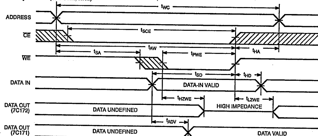
Write Cycle No. 1 (WE Controlled) [8]
