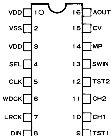
< 16DIP, 16SOP Top View >
