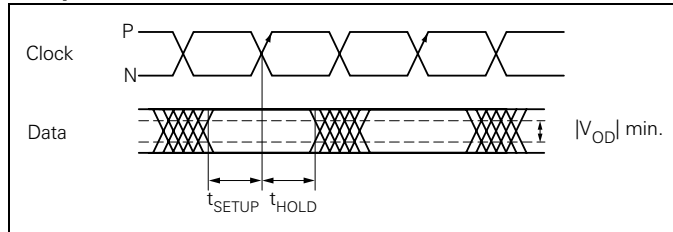
Figure 11. Measurement conventions for LVDS signals
