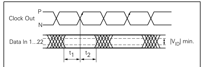
Figure 5. Timing diagrams
