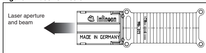
Figure 2. Laser emission
