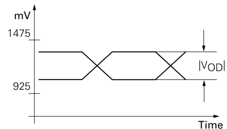
Figure 9. Output Levels
