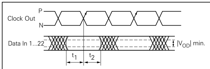
Figure 10. Timing diagrams
