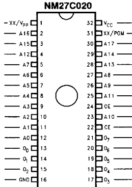
DIP Pin Configuration
