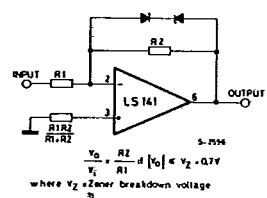
Fig. 28 - Clipping amplifier
