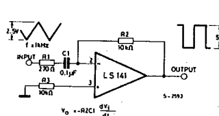
Fig. 30 - Simple differentiator
