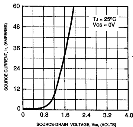
SOURCE-DRAIN DIODE FORWARD CHARACTERISTICS (TYPICAL) J1025
