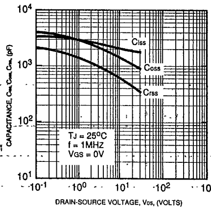
CAPACITANCE VS. DRAIN-SOURCE VOLTAGE (TYPICAL) J1025
