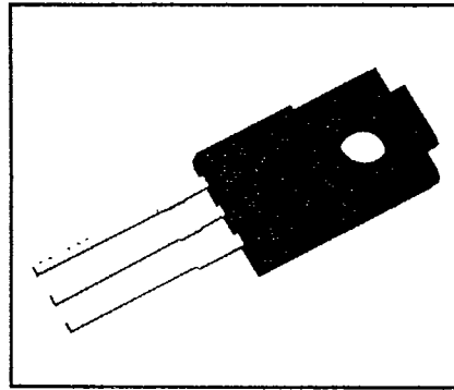
J1025 Single EXMOS™ MOSFET 20 Amperes/50 Volts
