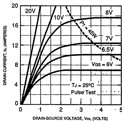
COMMON SOURCE OUTPUT CHARACTERISTICS (TYPICAL) J1025
