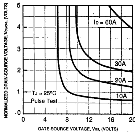
NORMALIZED DRAIN-SOURCE ON-STATE VOLTAGE (TYPICAL) J1025
