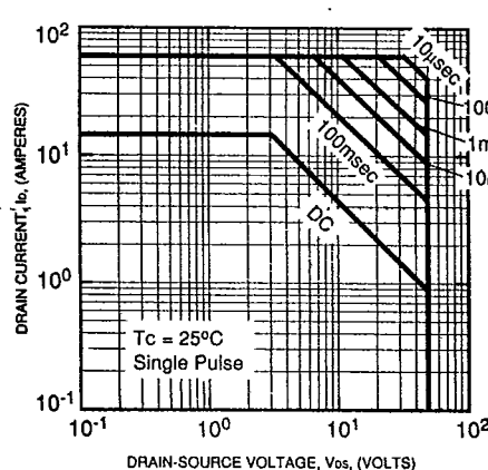
FORWARD BIAS SAFE OPERATING AREA (S.O.A.) J1025
