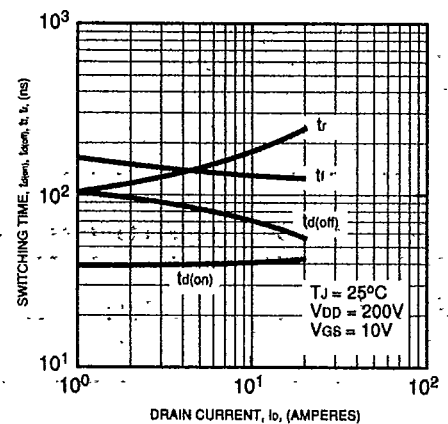
SWITCHING CHARACTERISTICS (TYPICAL) J1025
