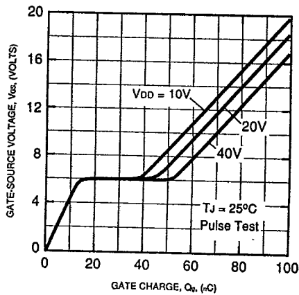
GATE CHARGE VS. V_{DS} AND V_{GS} (TYPICAL) J1025
