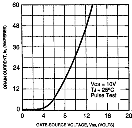
TRANSFER CHARACTERISTICS (TYPICAL) J1025
