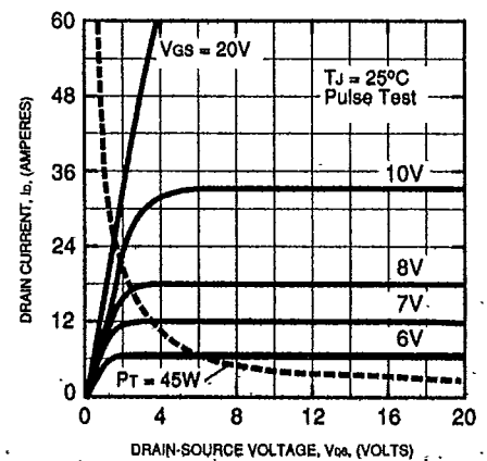
COMMON SOURCE OUTPUT CHARACTERISTICS (TYPICAL) J1025
