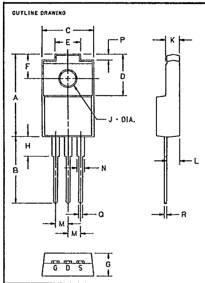
50 Volts J1025 Outline Drawing
