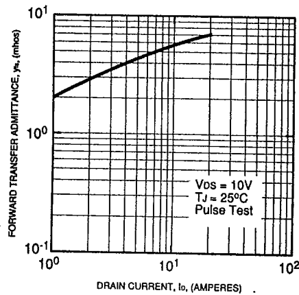
FORWARD TRANSFER ADMITTANCE VS. DRAIN CURRENT (TYPICAL) J1025
