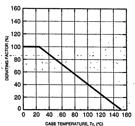
TEMPERATURE DERATING FACTOR OF SAFE OPERATING AREA (S.O.A.) J1025
