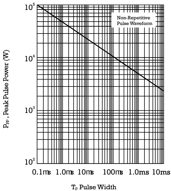
PULSE RATING CURVE
