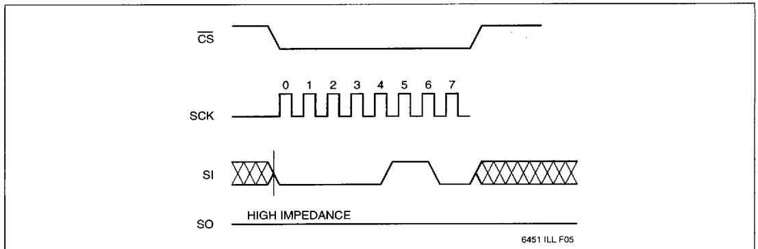
Figure 3. Write Enable Latch Sequence
