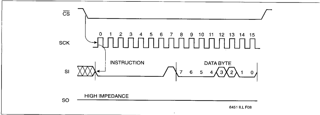
Figure 6. Write Status Register Operation Sequence
