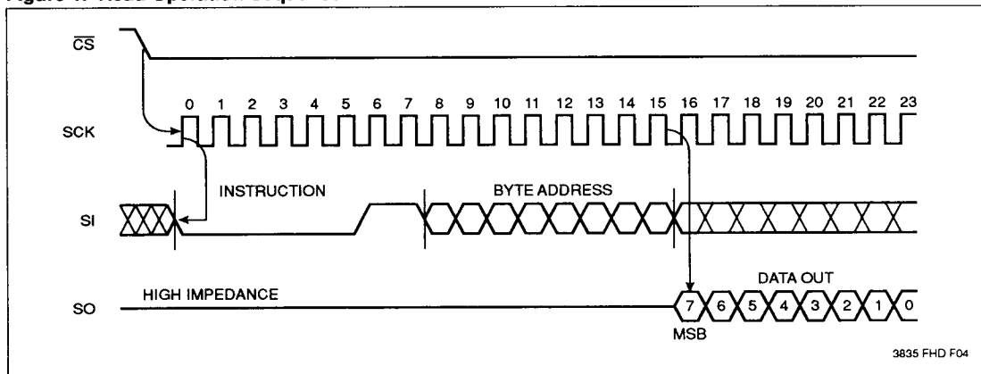
Figure 1. Read Operation Sequence
