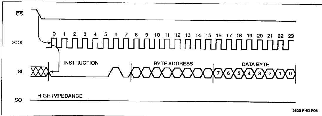
Figure 3. Write Operation Sequence
