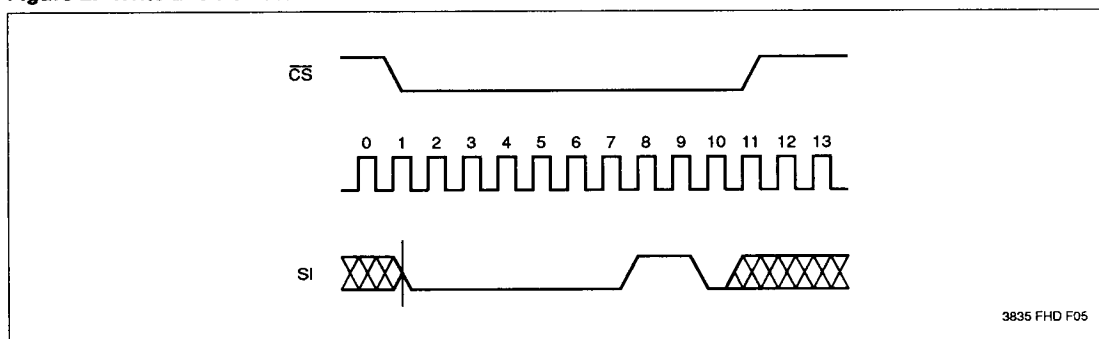
Figure 2. Write Enable Latch
