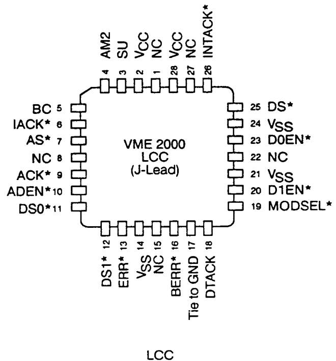
Figure 1. Pinout of VME 2000
