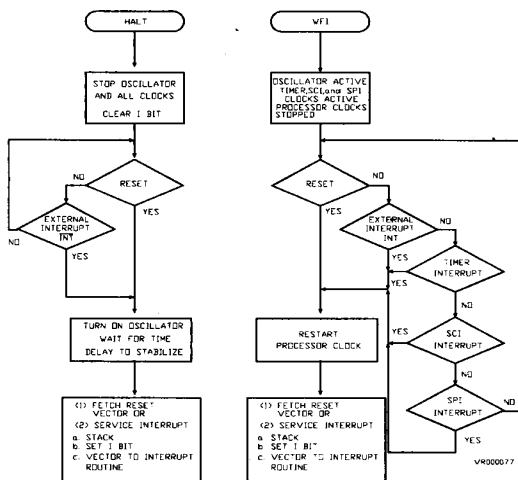
Figure 5.5 . HALT/WFI Flowchart
