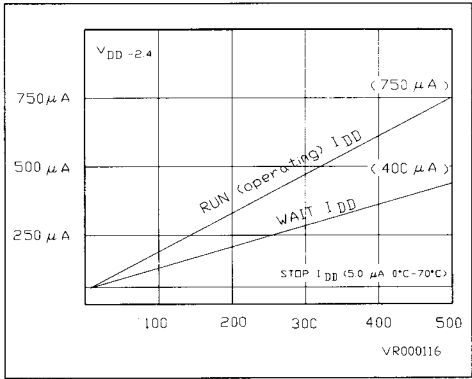
Figure 12.5. Maximum IDD vs Frequency for VDD = 2.4 Vdc
