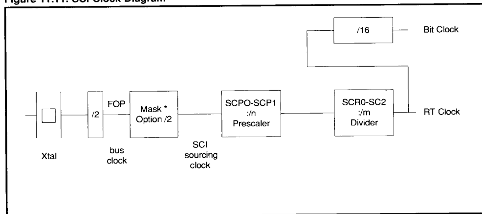
Figure 11.11. SCI Clock Diagram
