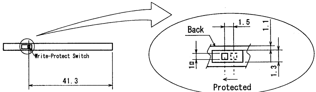
ENLARGEMENT OF THE WRITE-PROTECT SWITCH
