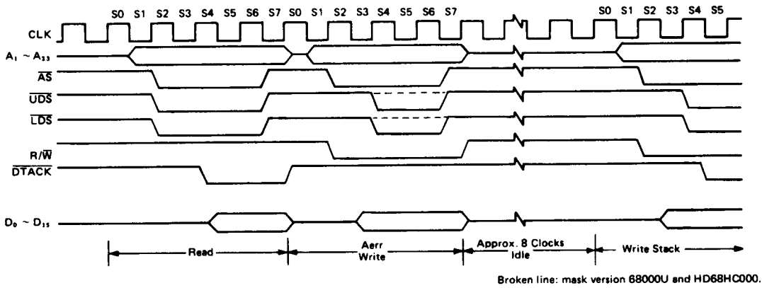
Figure 59 Address Error Timing
