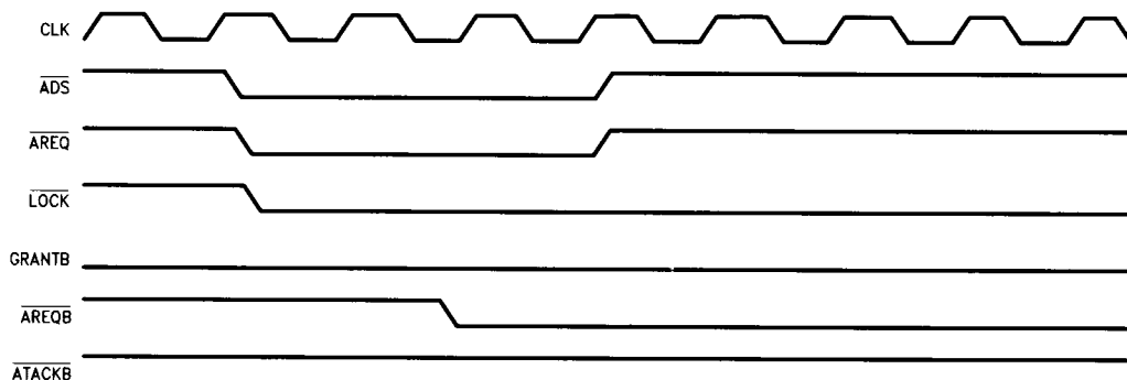
FIGURE 35. \overline{\text{LOCK}} Function
