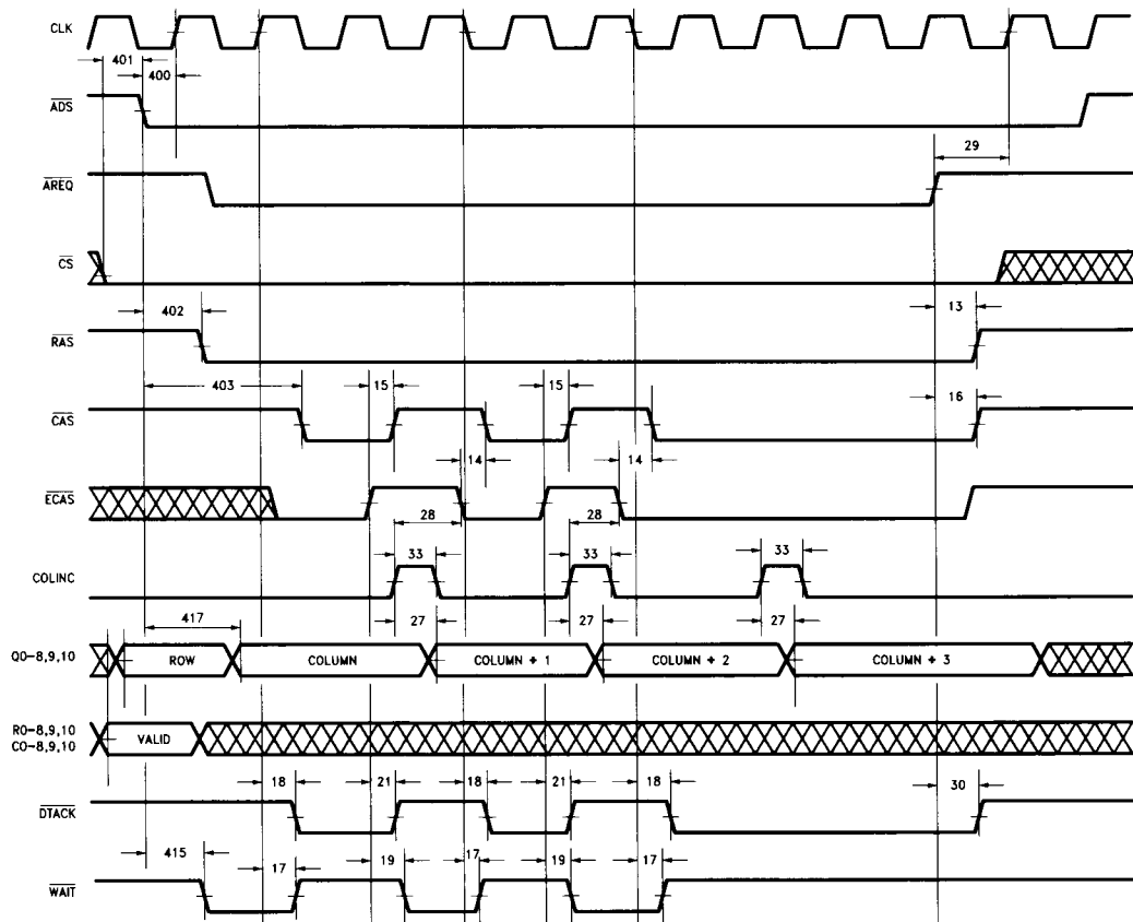
FIGURE 43. 400: COLINC Page/Static Column Access Timing
