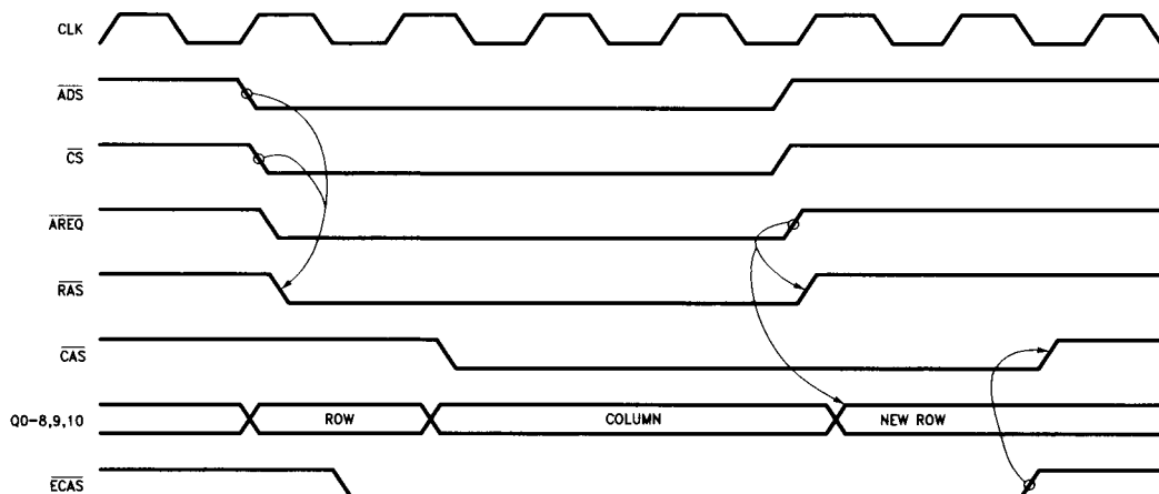
FIGURE 9b. Access Mode 1 Extending \overline{\text{CAS}}
