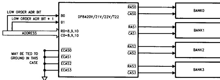
FIGURE 29a. DRAM Array Setup for 4 Banks Using Error Scrubbing (C6, C5, C4 = 0, 1, 0 during Programming)
