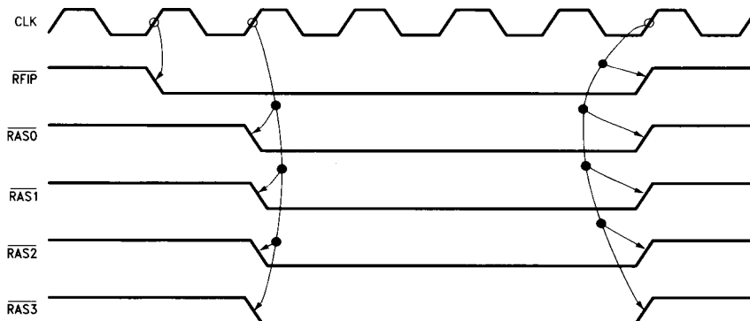
FIGURE 16. Conventional RAS Refresh
