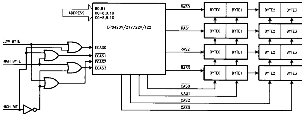
FIGURE 26d. 8 Bank DRAM Array for 16-Bit System (C6, C5, C4 = 1, 1, 0 during Programming)
