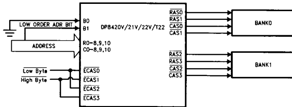
FIGURE 28b. DRAM Array Setup for Address Pipelining with 2 Banks (C6, C5, C4 = 1, 0, 1 or C6, C5, C4 = 0, 0, 1 (Also Allowing Error Scrubbing) during Programming)
