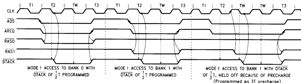
FIGURE 25. Guaranteeing \overline{RAS} Precharge ( DTACK is Sampled at the "T2" Falling Clock Edge)
