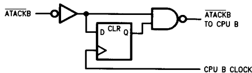
C. Synchronize \overline{ATACKB} to CPU B Clock. This is useful if CPU B runs asynchronous to the DP8422V, DP84T22.
