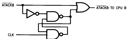
A. Extend \overline{ATACK} to \frac{1}{2}T ( \frac{1}{2} Clock) after \overline{RAS} goes low.
