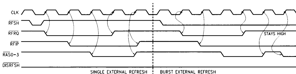
FIGURE 15a. Externally Controlled Single and Burst Refresh with Refresh Request ( \overline{RFRQ} ) Output (2 Periods of \overline{RAS} Low during Refresh Programmed)
