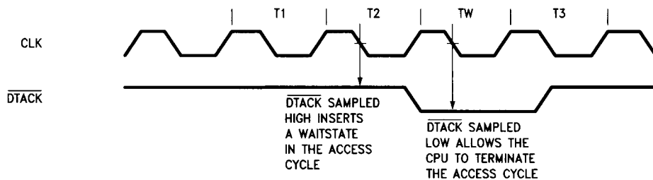
FIGURE 23. \overline{DTACK} Type Output
