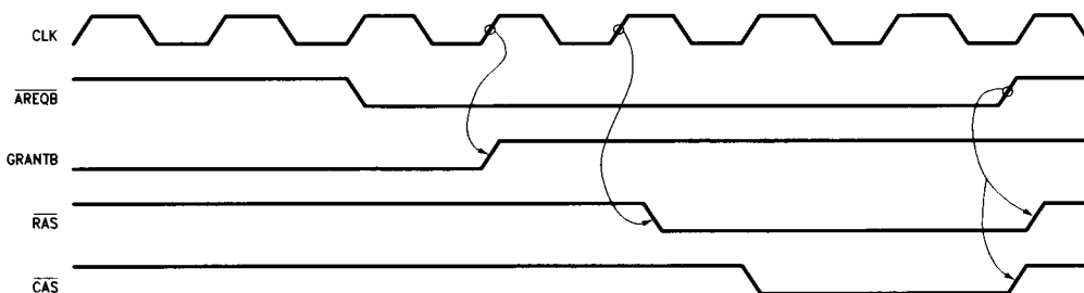
FIGURE 32c. Delayed Port B Access
