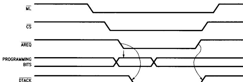
FIGURE 7. \overline{CS} Access Programming
