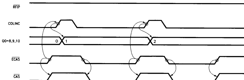
FIGURE 10. Column Increment
