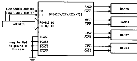
FIGURE 28a. DRAM Array Setup for 4 Banks Using Address Pipelining (C6, C5, C4 = 1, 1, 1 or C6, C5, C4 = 0, 1, 0 (Also Allowing Error Scrubbing) during Programming)
