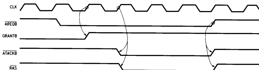
FIGURE 33b. Delayed Port B Access
