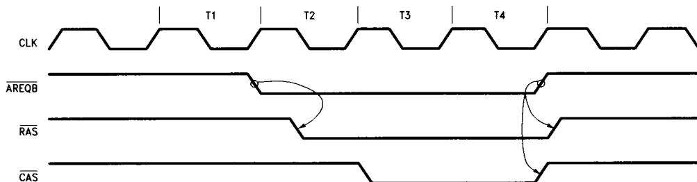
FIGURE 32b. Access Request for Port B
