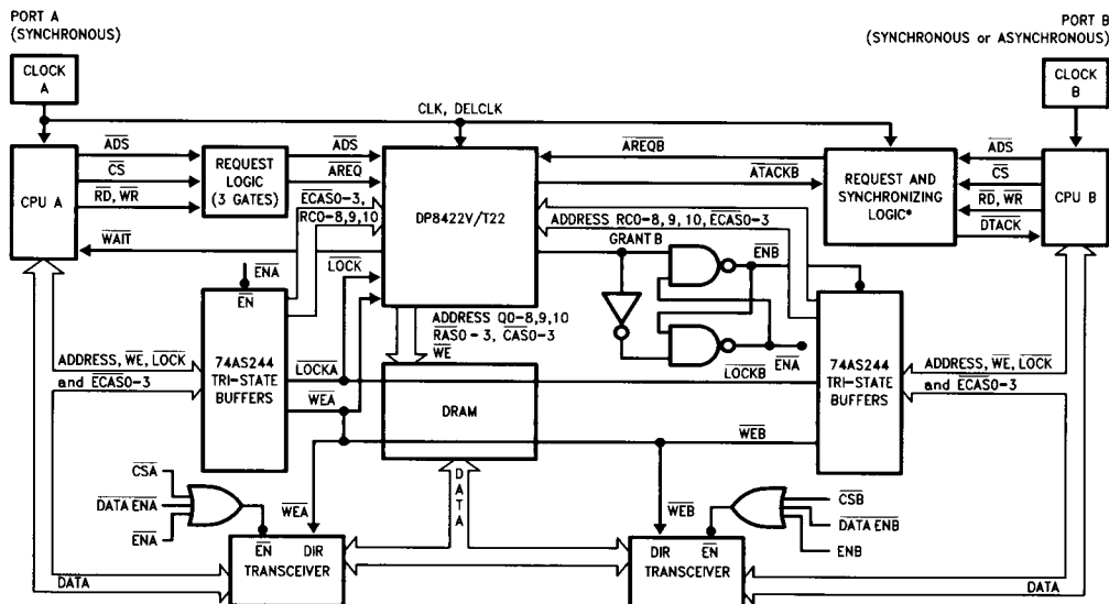
FIGURE 34a. Dual Accessing with the DP8422V, DP84T22 (System Block Diagram)
