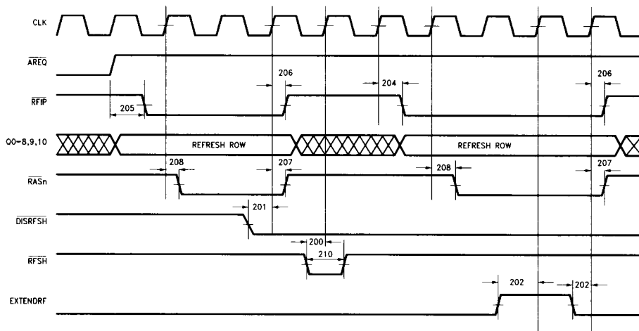
FIGURE 39. 200: Refresh Timing
