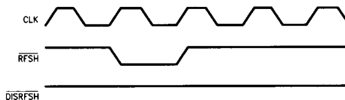
FIGURE 20a. Clearing the Refresh Address Counter
