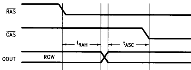
FIGURE 31. t_{RAH} and t_{ASC}
