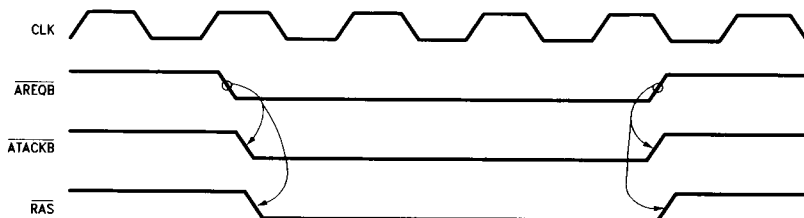
FIGURE 33a. Non-Delayed Port B Access
