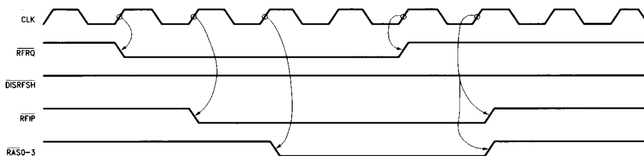
FIGURE 15b. Automatic Internal Refresh with Refresh Request (3T of \overline{RAS} Low during Refresh Programmed)
