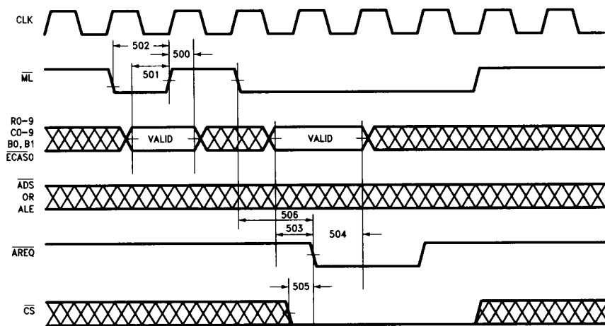
FIGURE 44. 500: Programming
