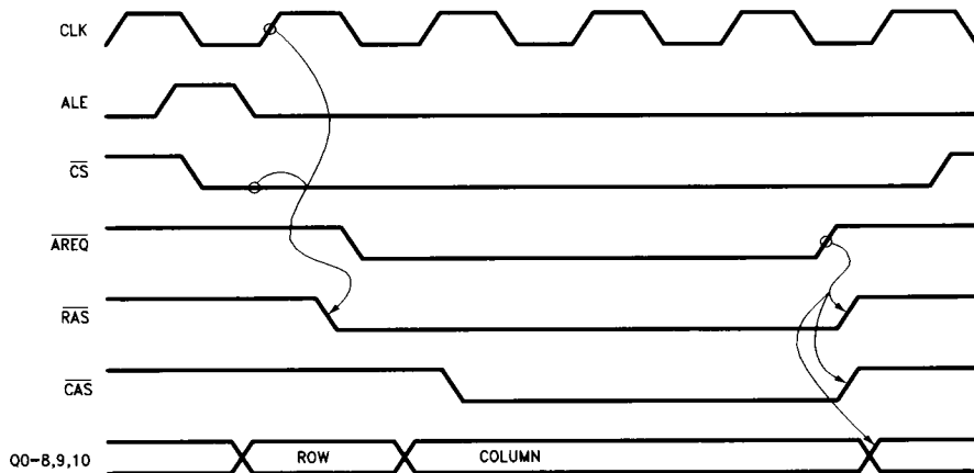
FIGURE 8a. Access Mode 0
