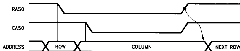
FIGURE 11a. Non-Address Pipelined Mode
