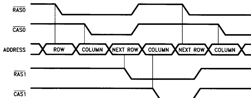
FIGURE 11b. Address Pipelined Mode
