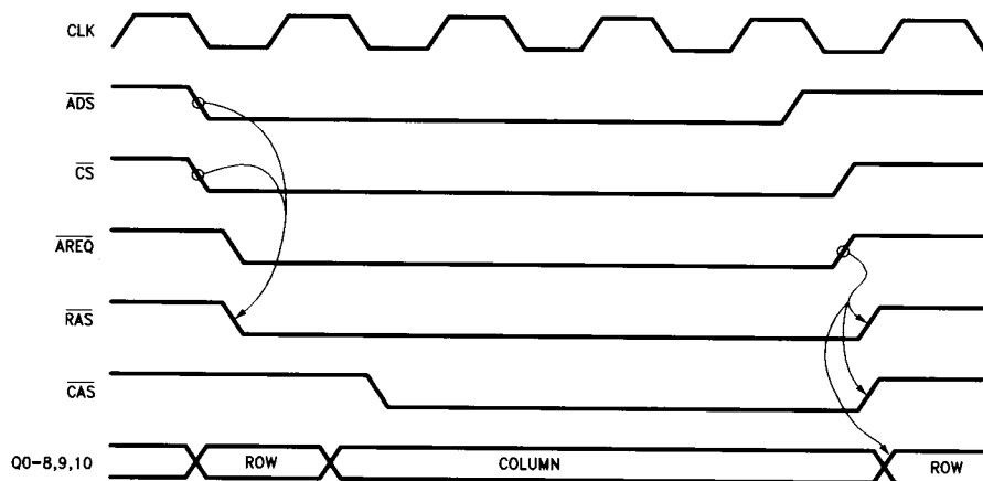
FIGURE 8b. Access Mode 1
