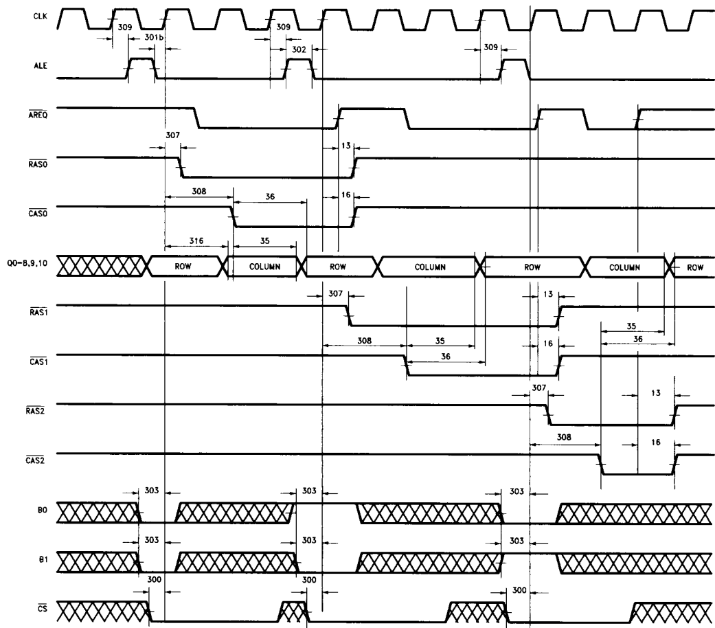
FIGURE 41. 300: Mode 0 Interleaving
