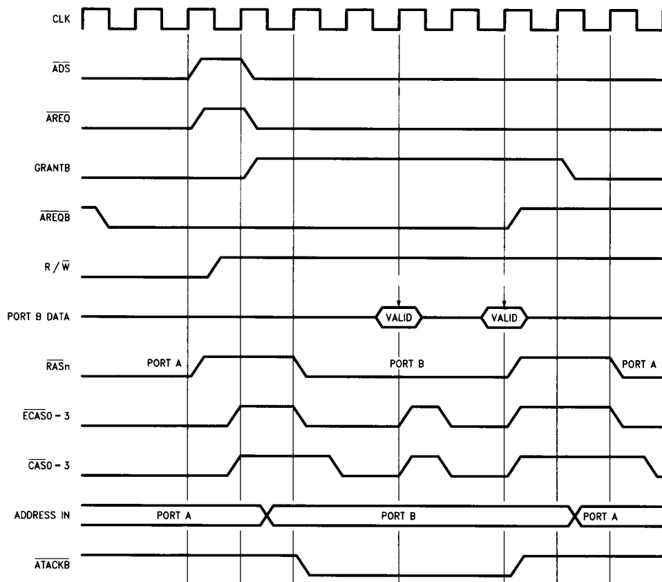
FIGURE 34b. Wait States during a Port B Access
