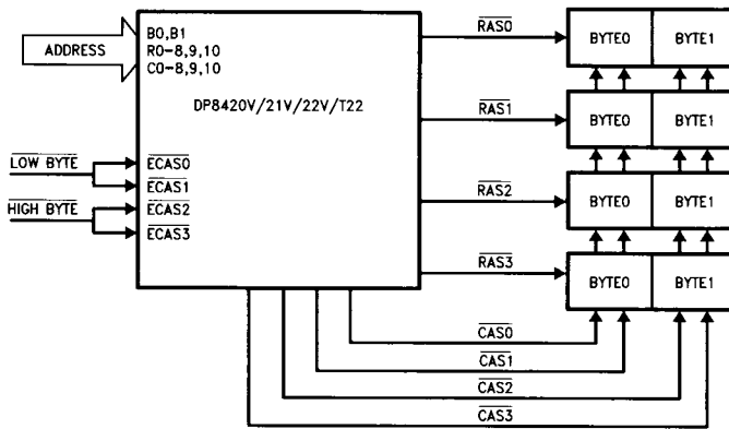
FIGURE 26c. DRAM Array Setup for 16-Bit System (C6, C5, C4 = 1, 1, 0 during Programming)
