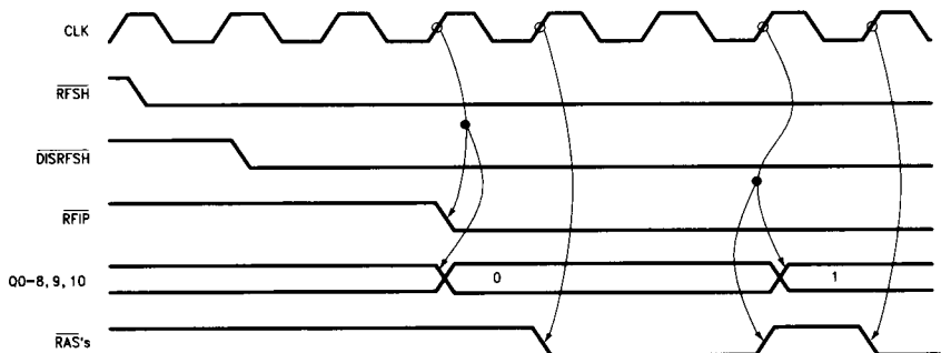
FIGURE 20b. Clearing the Refresh Counter during Burst
