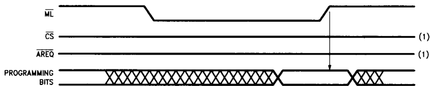
FIGURE 6. \overline{ML} Only Programming
