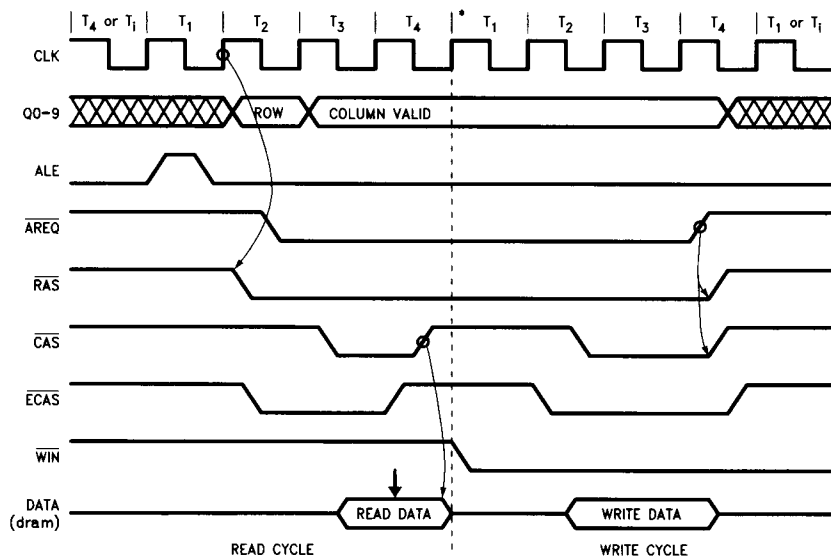
FIGURE 9c. Read-Modify-Write Access Cycle
