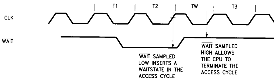
FIGURE 22. \overline{\text{WAIT}} Type Output
