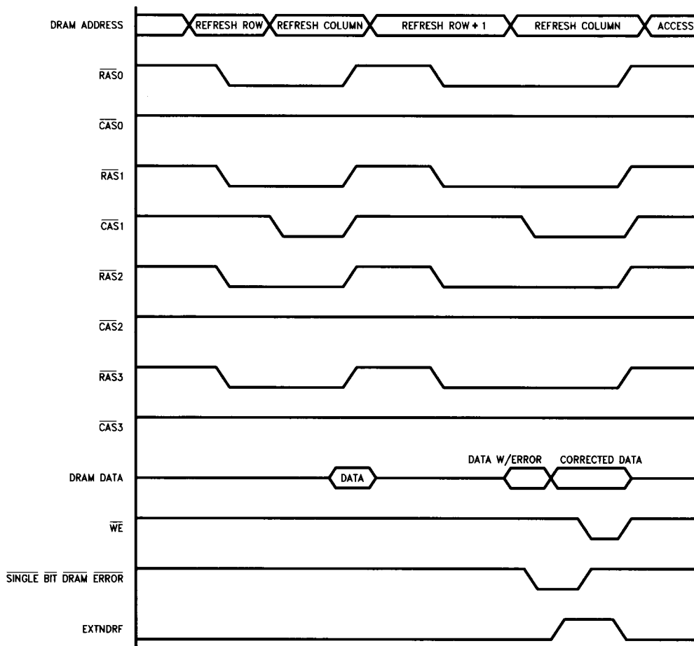
FIGURE 18. Error Scrubbing during Refresh
