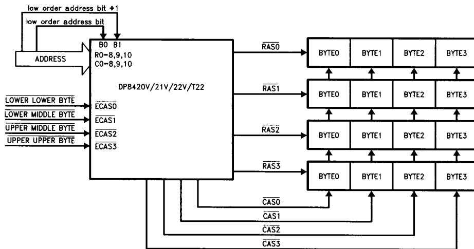
FIGURE 27. Memory Interleaving (C6, C5, C4 = 1, 1, 0 during Programming)
