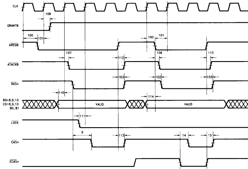
FIGURE 37. 100: Dual Access Port B
