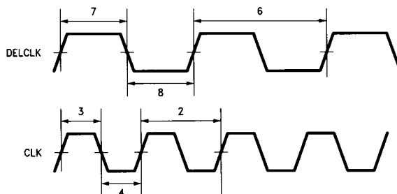
FIGURE 36. Clock, DELCLK Timing
