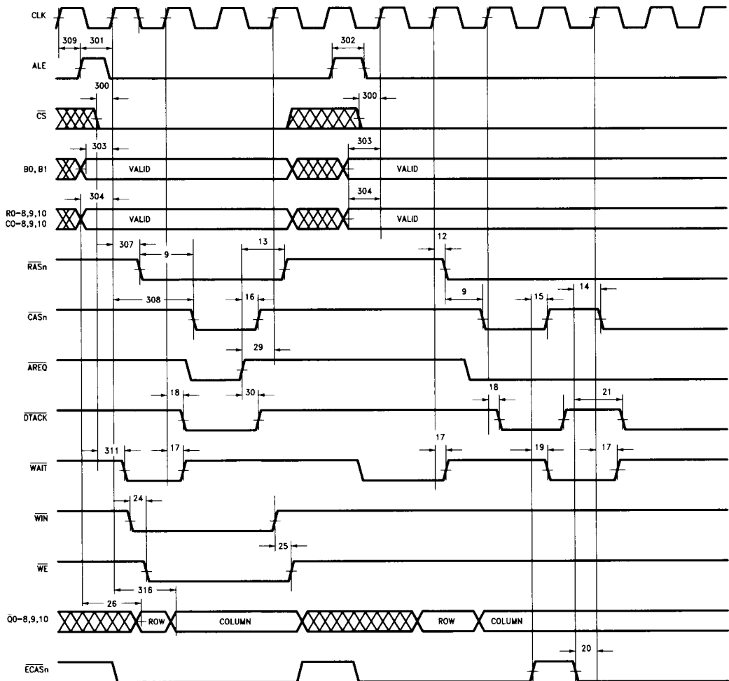
FIGURE 40. 300: Mode 0 Timing
