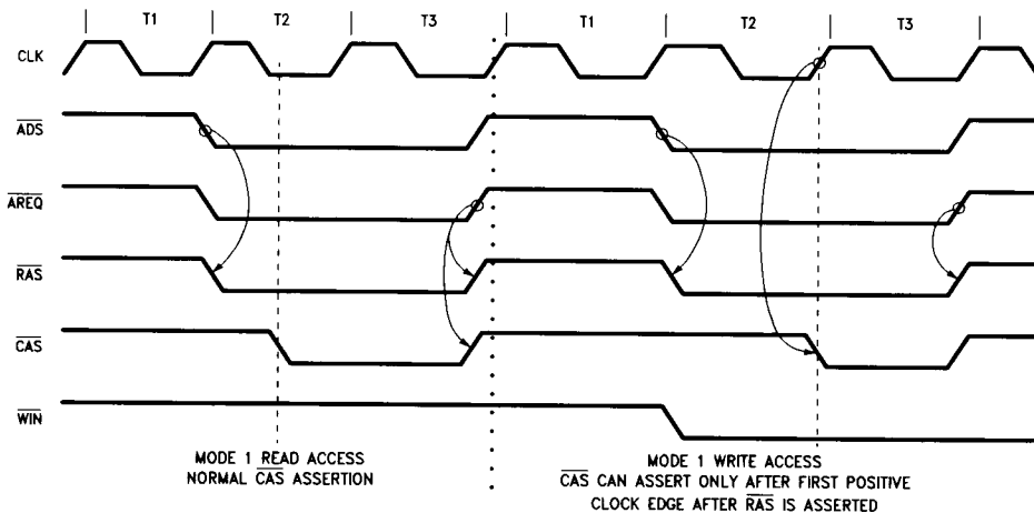
FIGURE 12b. Mode 1 Delay \overline{\text{CAS}}
