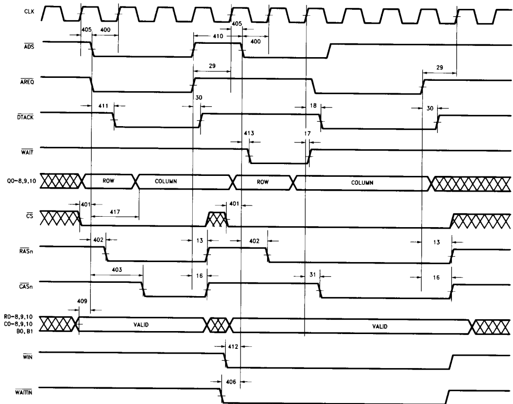
FIGURE 42. 400: Mode 1 Timing
