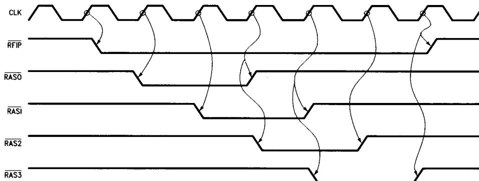
FIGURE 17. Staggered RAS Refresh
