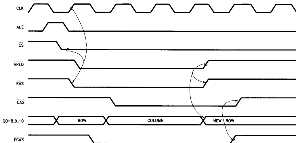
FIGURE 9a. Access Mode 0 Extending \overline{\text{CAS}}
