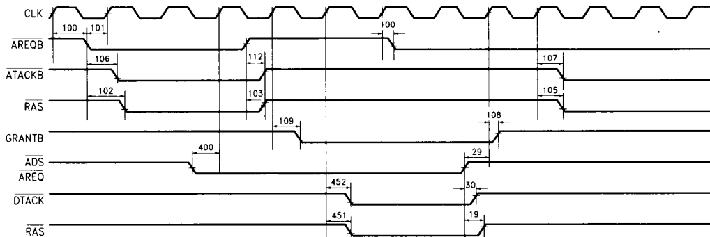
FIGURE 38. 100: Port A and Port B Dual Access
