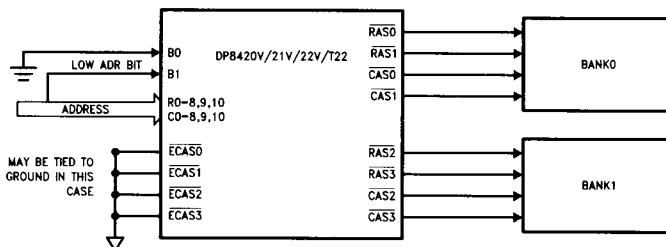
FIGURE 29b. DRAM Array Setup for Error Scrubbing with 2 Banks (C6, C5, C4 = 0, 0, 1 during Programming)
