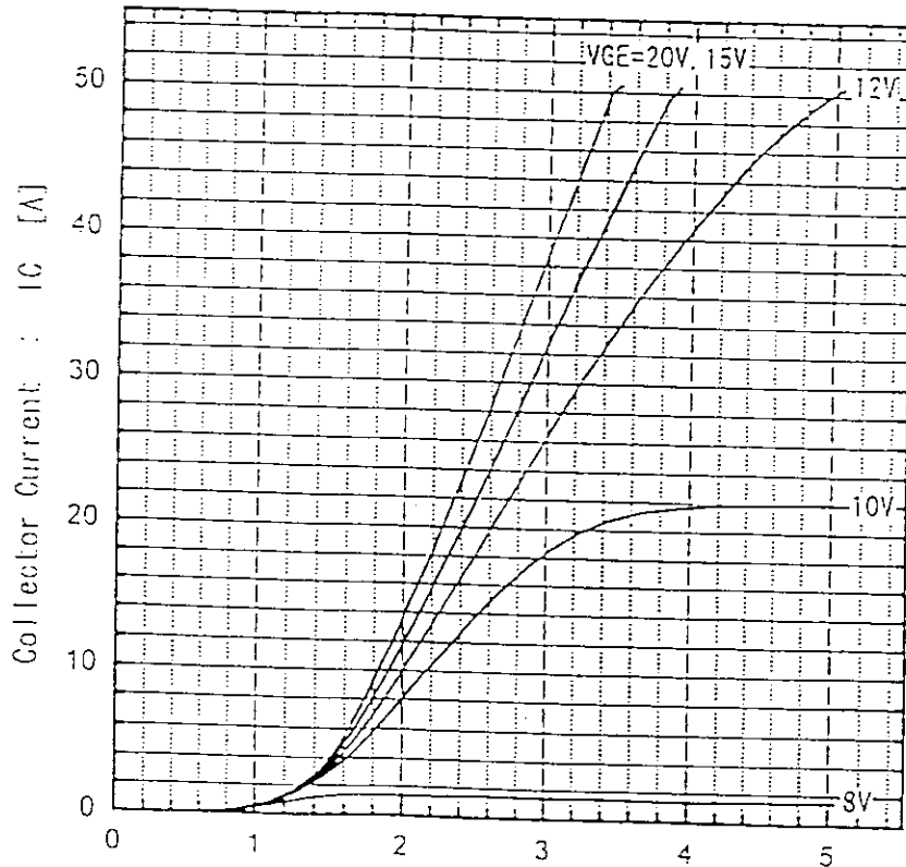
Collector Current vs. Collector-Emitter Voltage T_j = 25^\circ\text{C}
