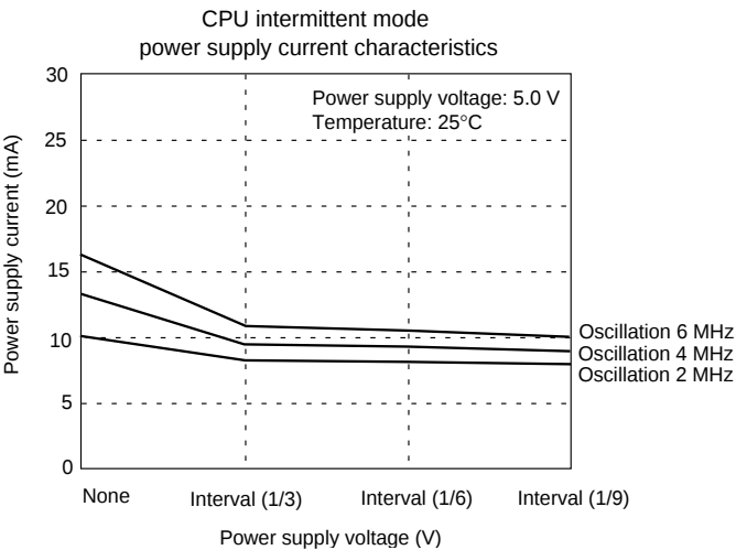
CPU intermittent mode power supply current characteristics
