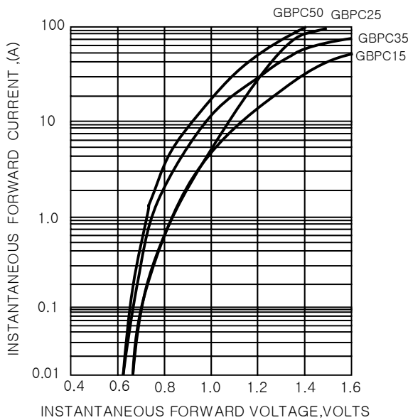
FIG.3-TYPICAL FORWARD CHARACTERISTICS
