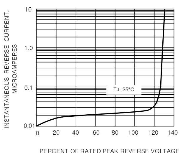
FIG.4-TYPICAL REVERSE CHARACTERISTICS
