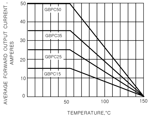
FIG.2-DEATING CURVE OUTPUT RECTIFIED CURRENT
