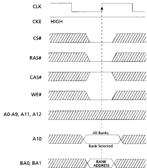
FIGURE 20: PRECHARGE Command
