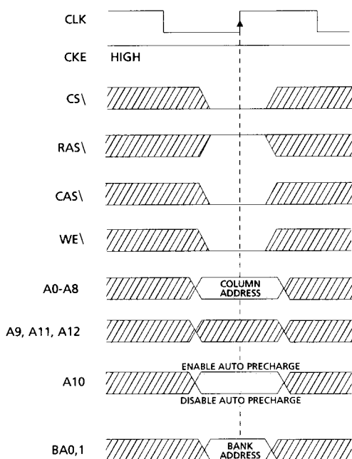
FIGURE 13: WRITE Command
