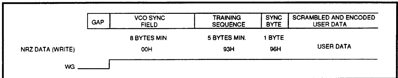
FIGURE 9: Hard Sector Write Sequence
