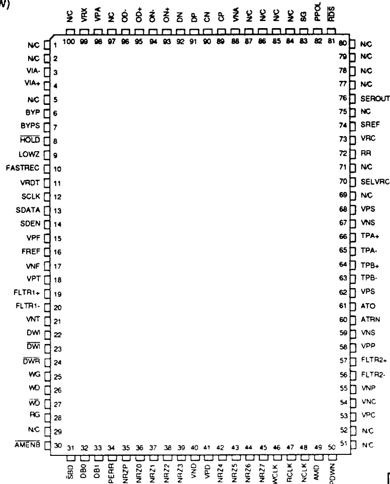
100-Lead QFP
