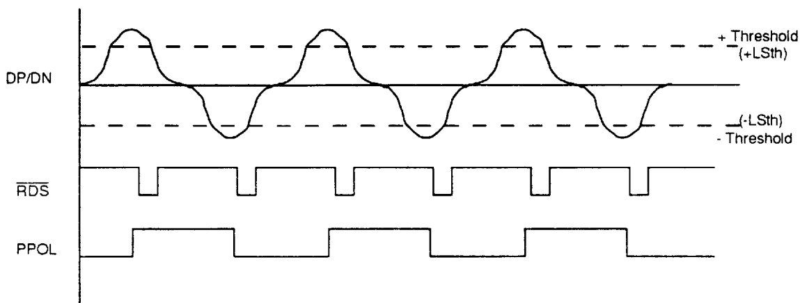
FIGURE 6: \overline{RDS} and PPOL vs. DP/DN Relationship
