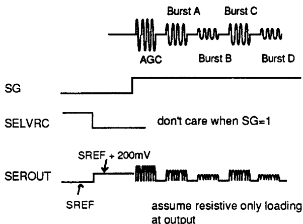
FIGURE 5: Sevo Function Diagram
