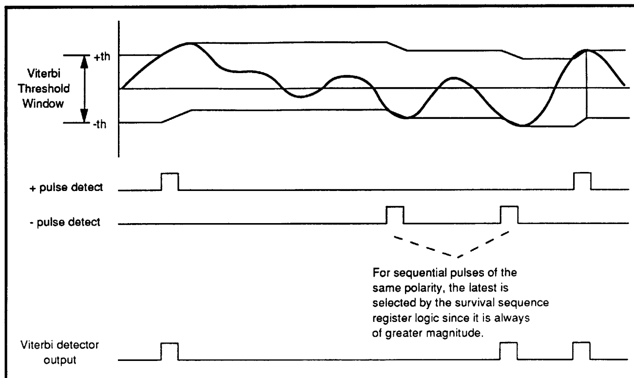
FIGURE 1: Viterbi Detection
